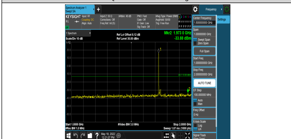
Band4-10MHz-16QAM-20175-1RB#0-Range4:1000~2000MHz
