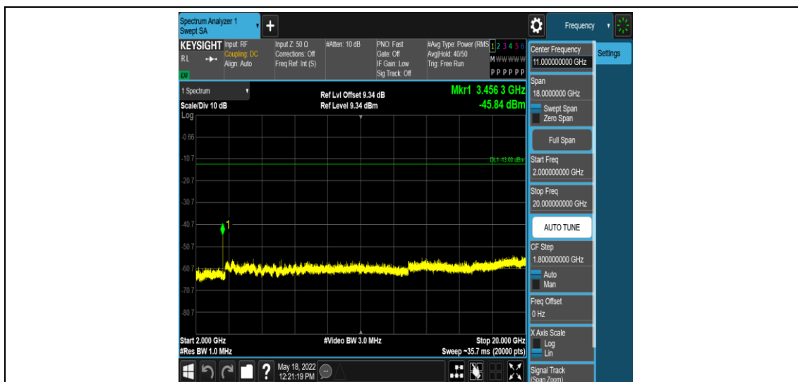
Band4-10MHz-16QAM-20175-1RB#0-Range5:2000~20000MHz
