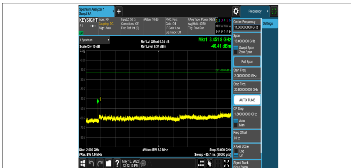
Band4-15MHz-QPSK-20175-1RB#0-Range5:2000~20000MHz
