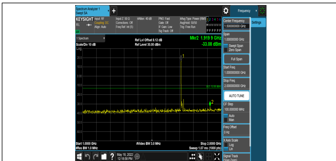
Band4-10MHz-16QAM-20000-1RB#0-Range4:1000~2000MHz
