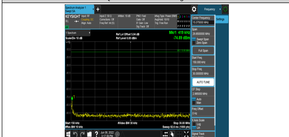
Band40-5MHz-16QAM-39200-1RB#0-Range2:0.15~30MHz
