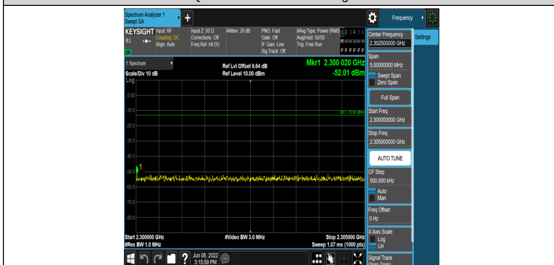
Band40-5MHz-QPSK-39200-1RB#0-Range8:2300~2305MHz
