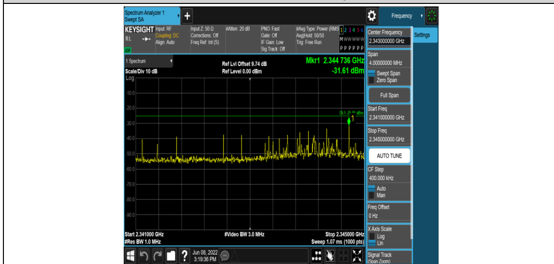
Band40-5MHz-16QAM-39200-1RB#0-Range13:2341~2345MHz
