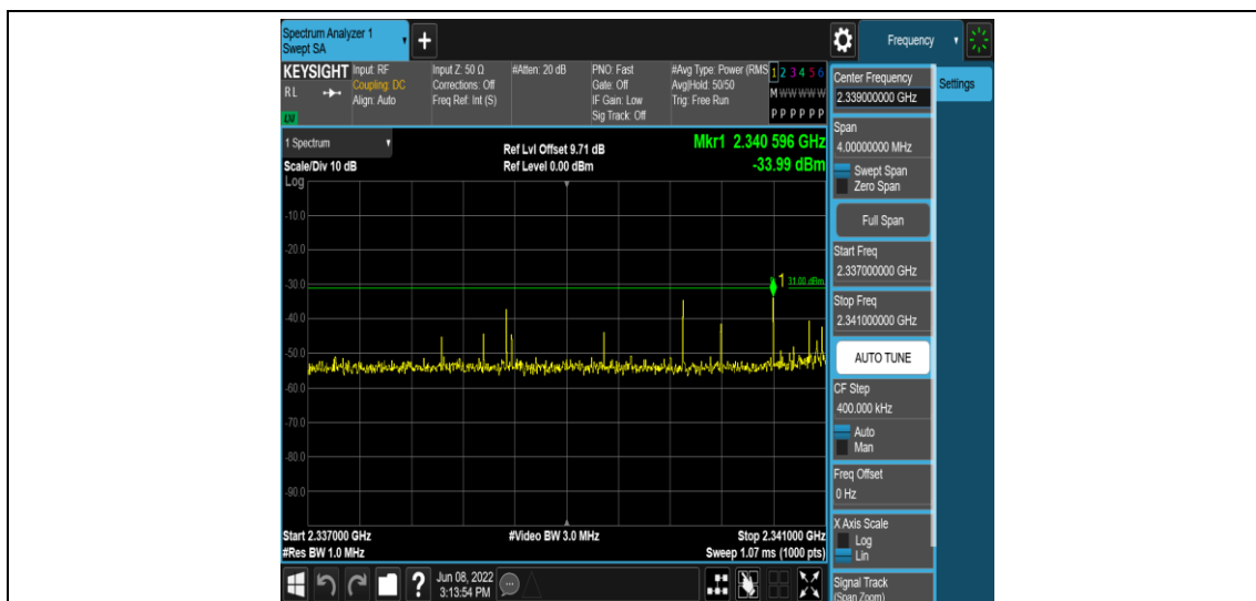
Band40-5MHz-16QAM-39175-1RB#0-Range12:2337~2341MHz
