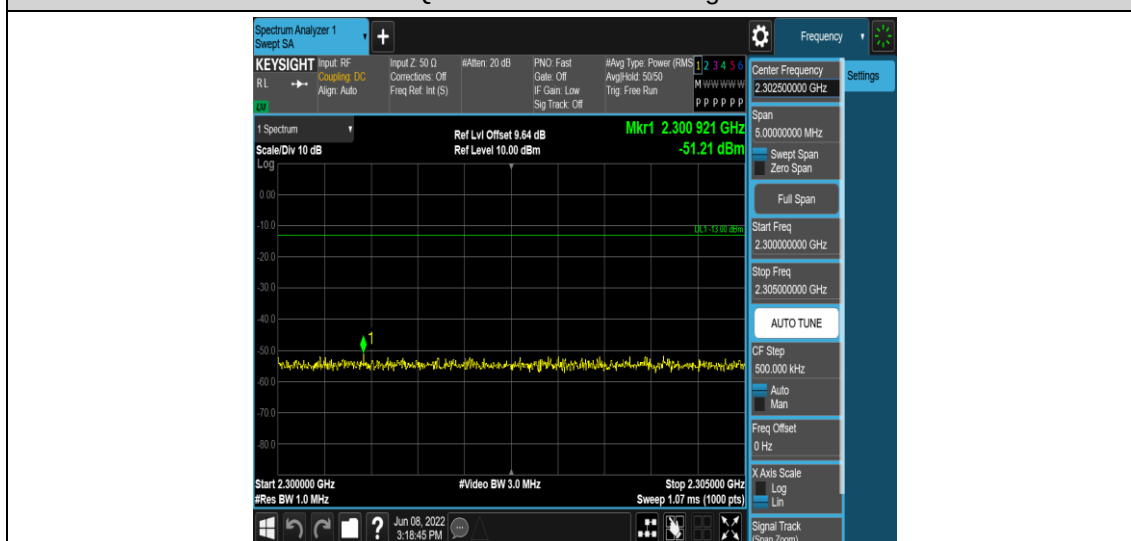
Band40-5MHz-16QAM-39200-1RB#0-Range8:2300~2305MHz
