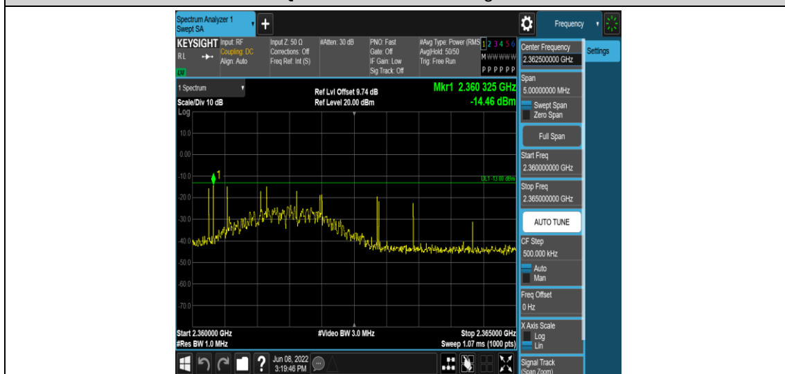
Band40-5MHz-16QAM-39200-1RB#0-Range14:2360~2365MHz
