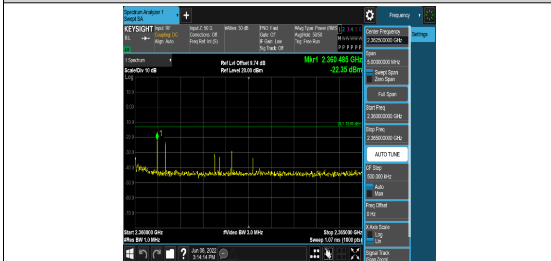
Band40-5MHz-16QAM-39175-1RB#0-Range14:2360~2365MHz
