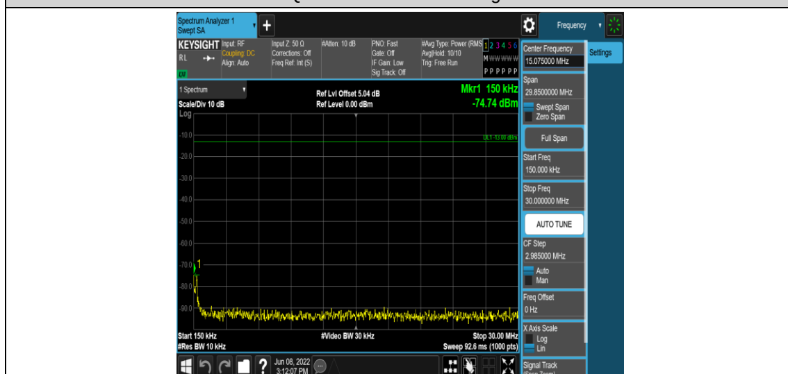
Band40-5MHz-16QAM-39175-1RB#0-Range2:0.15~30MHz
