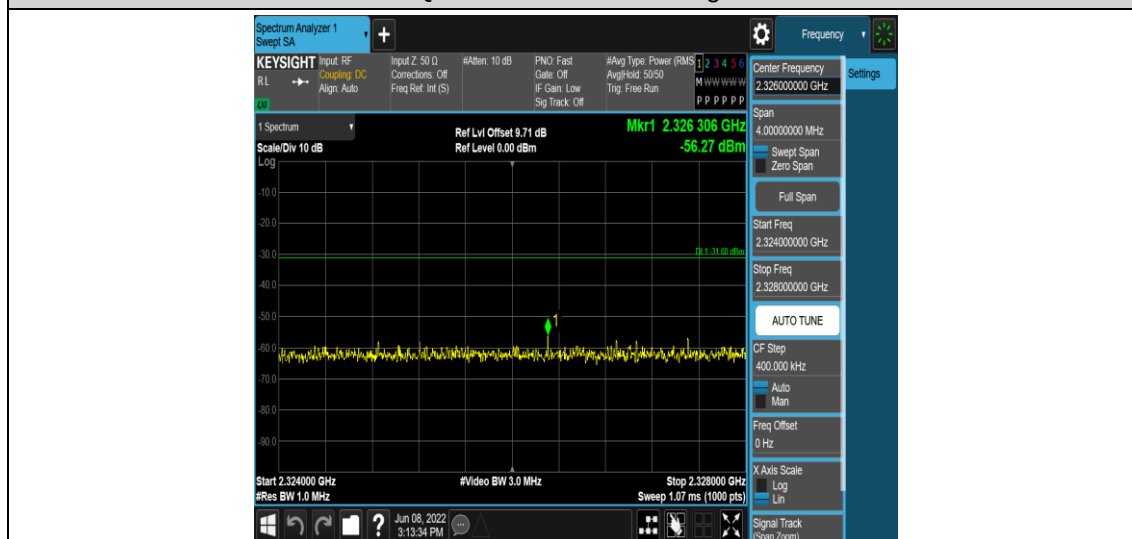
Band40-5MHz-16QAM-39175-1RB#0-Range10:2324~2328MHz
