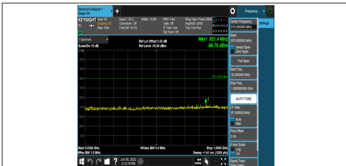
Band40-5MHz-16QAM-39175-1RB#0-Range3:30~1000MHz
