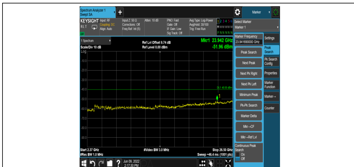
Band40-5MHz-16QAM-39200-1RB#0-Range15:2365~26500MHz
