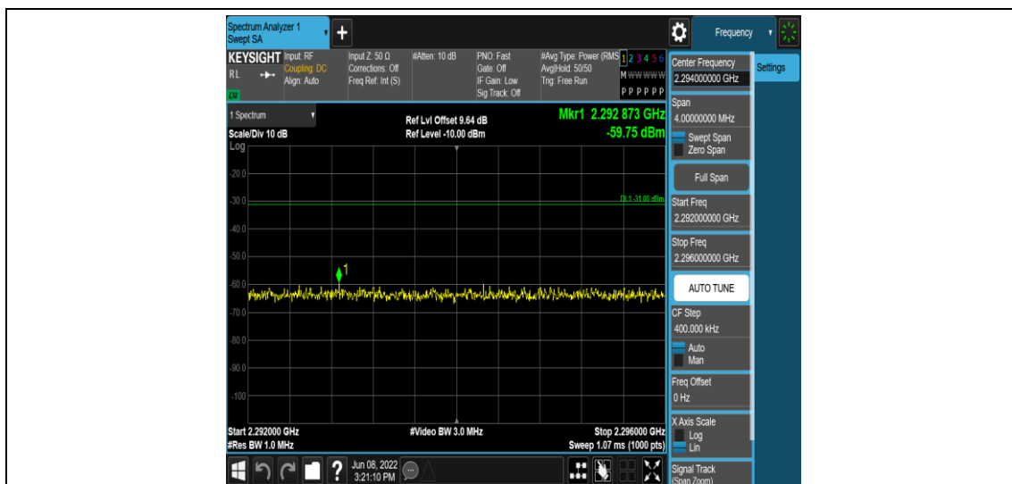
Band40-5MHz-QPSK-39225-1RB#0-Range6:2292~2296MHz
