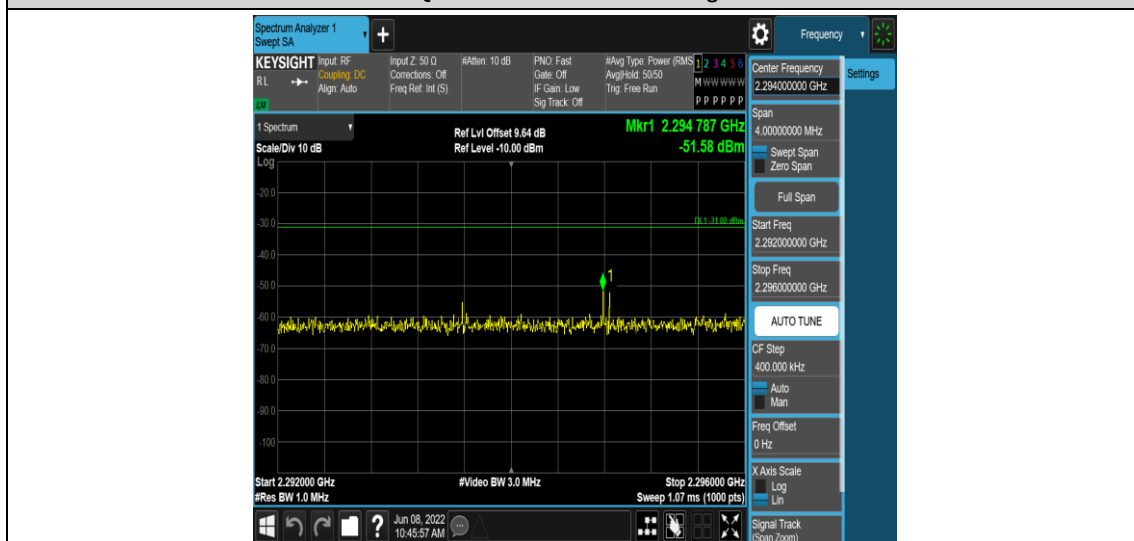
Band40-5MHz-16QAM-38775-1RB#0-Range6:2292~2296MHz
