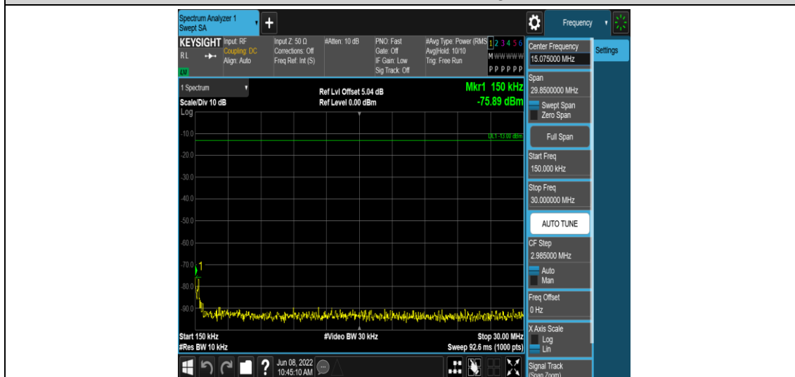
Band40-5MHz-16QAM-38775-1RB#0-Range2:0.15~30MHz
