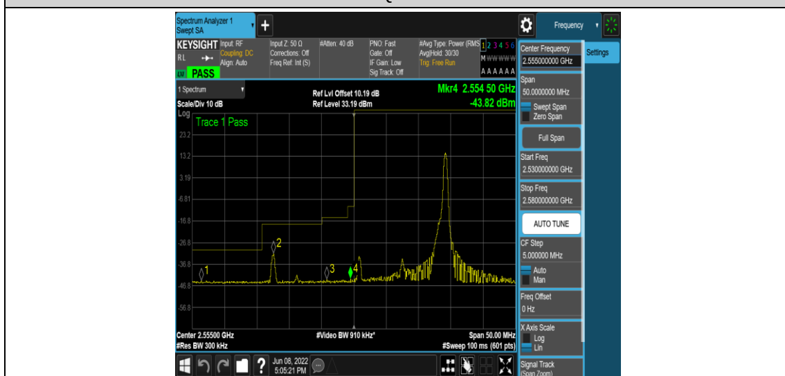
Band41-15MHz-QPSK-40315-1RB#74
