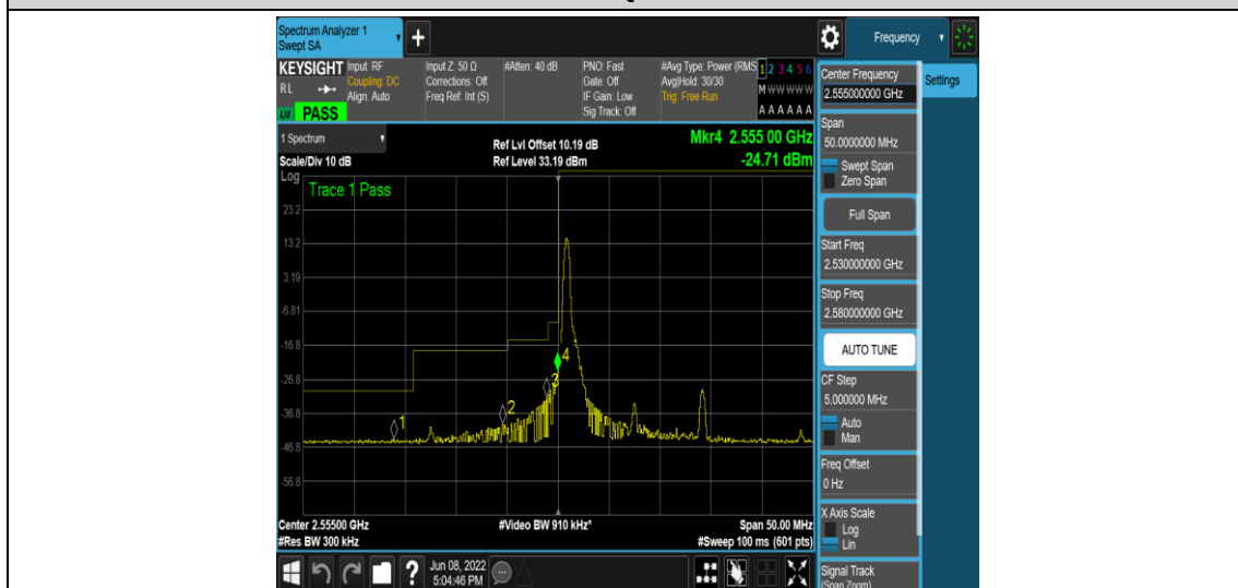
Band41-15MHz-QPSK-40315-1RB#0
