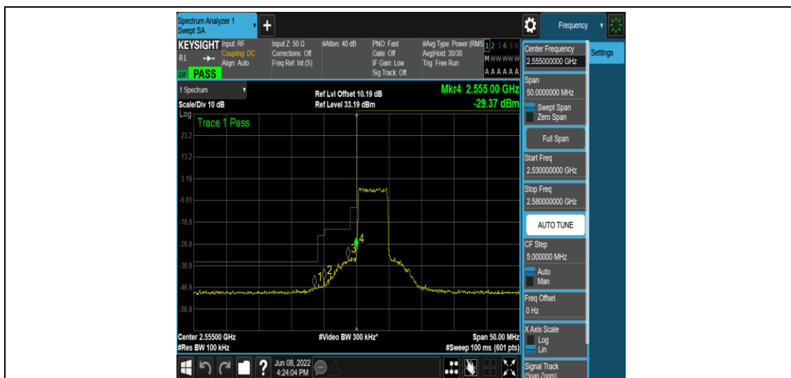
Band41-5MHz-16QAM-40265-25RB#0
