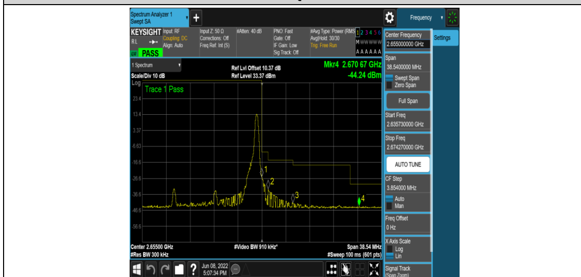
Band41-15MHz-16QAM-41165-1RB#74
