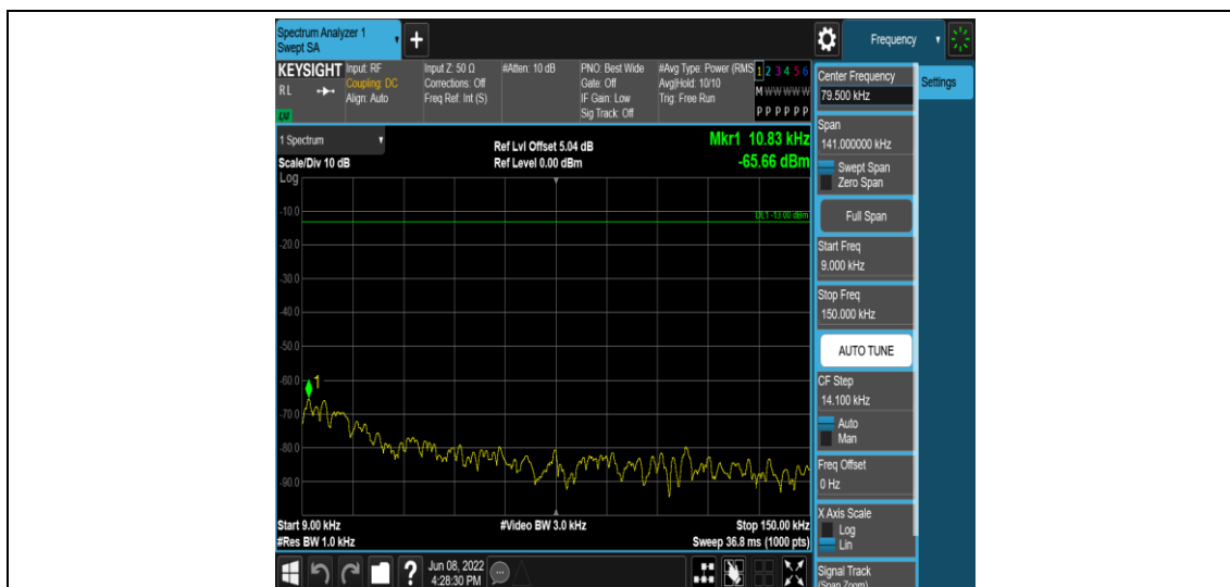
Band41-5MHz-QPSK-40740-1RB#0-Range1:0.009~0.15MHz
