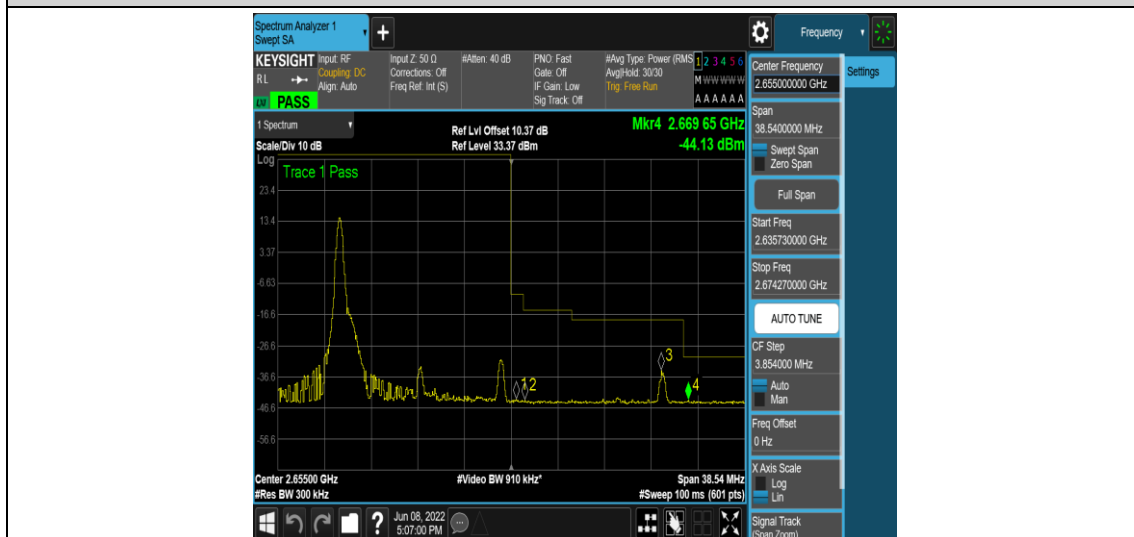
Band41-15MHz-16QAM-41165-1RB#0
