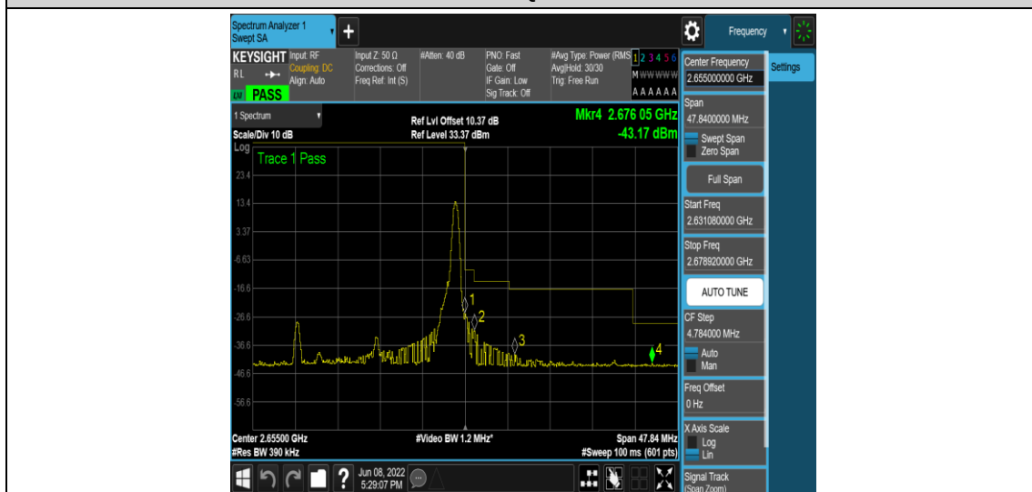
Band41-20MHz-16QAM-41140-1RB#99
