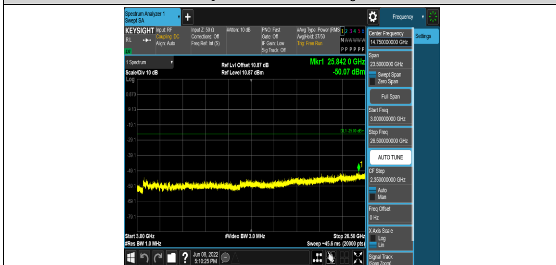
Band41-15MHz-16QAM-40315-1RB#0-Range5:3000~26500MHz
