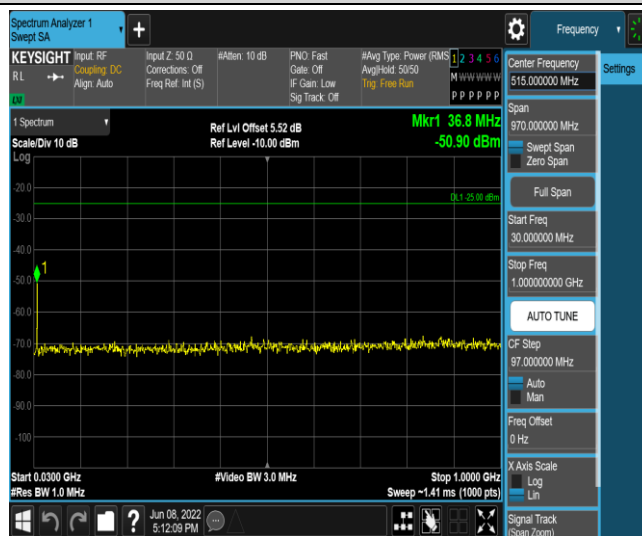
Band41-15MHz-16QAM-40740-1RB#0-Range3:30~1000MHz
