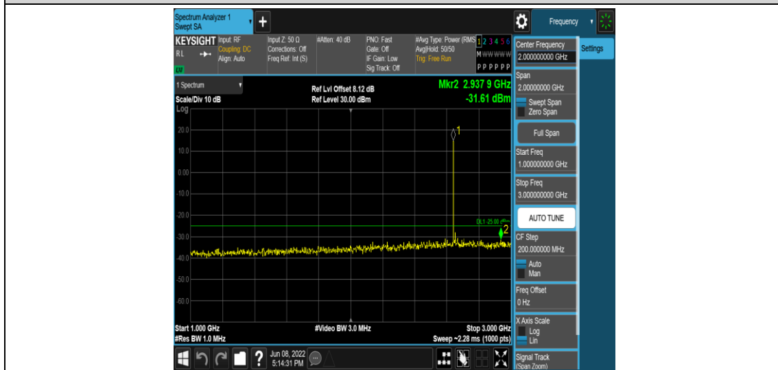
Band41-15MHz-16QAM-41165-1RB#0-Range4:1000~3000MHz
