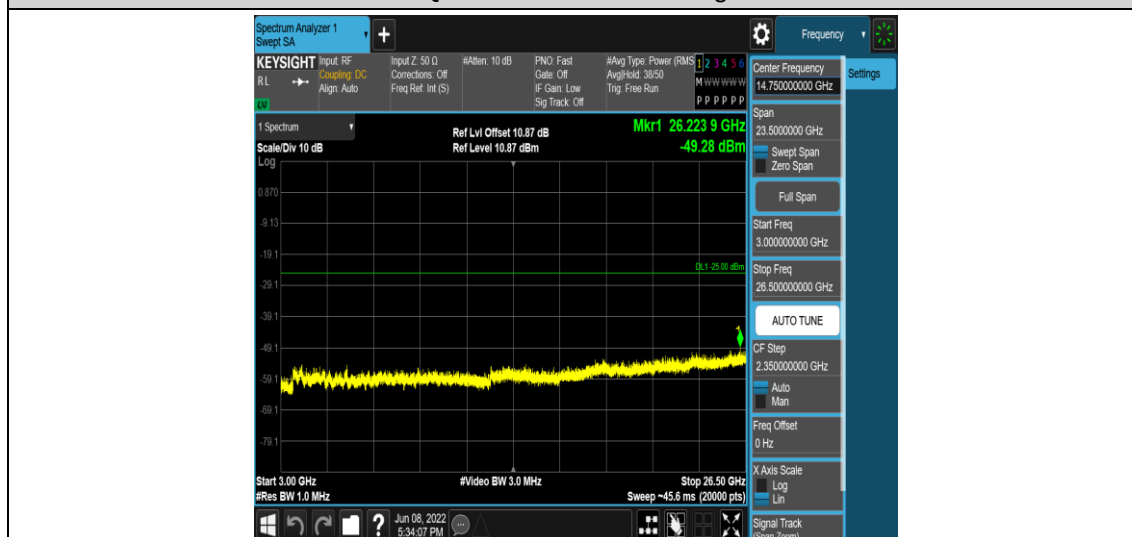
Band41-20MHz-16QAM-40740-1RB#0-Range5:3000~26500MHz
