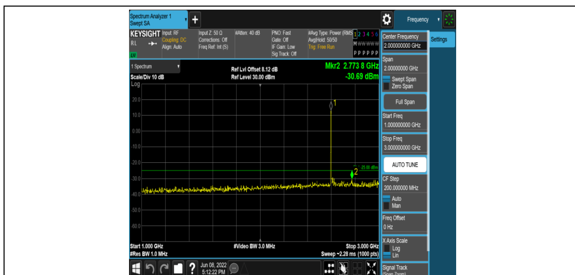
Band41-15MHz-16QAM-40740-1RB#0-Range4:1000~3000MHz
