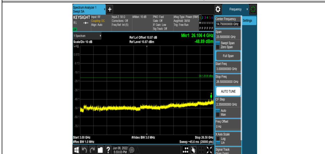
Band41-20MHz-QPSK-40740-1RB#0-Range5:3000~26500MHz
