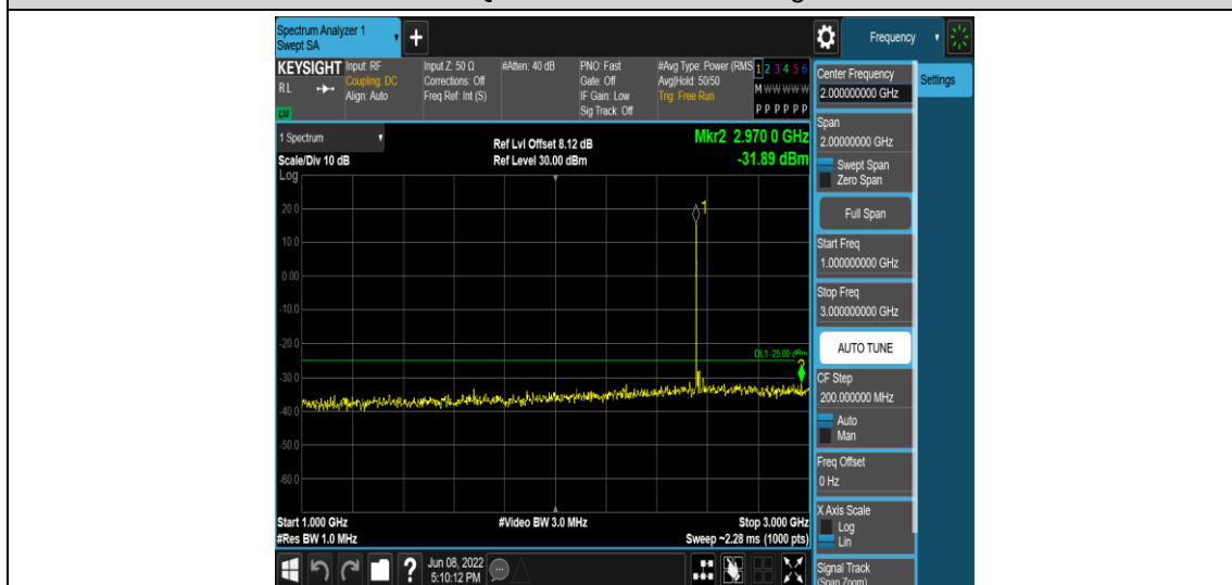
Band41-15MHz-16QAM-40315-1RB#0-Range4:1000~3000MHz
