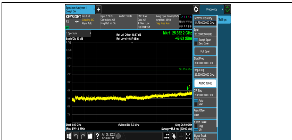
Band41-15MHz-QPSK-41165-1RB#0-Range5:3000~26500MHz
