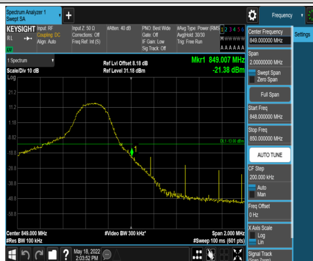
Band5-5MHz-16QAM-20625-1RB#24
