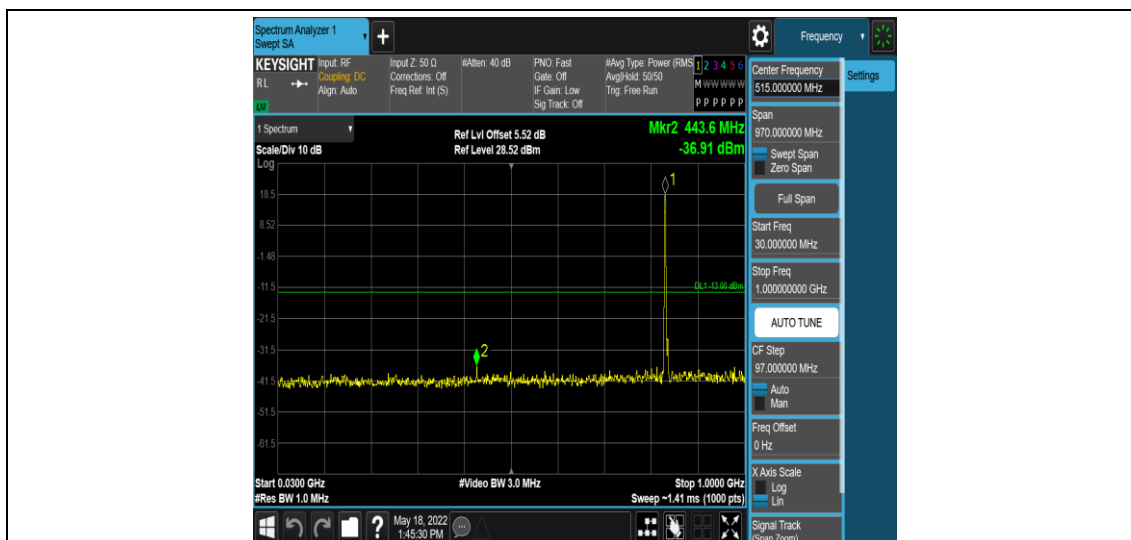
Band5-3MHz-QPSK-20525-1RB#0-Range3:30~1000MHz
