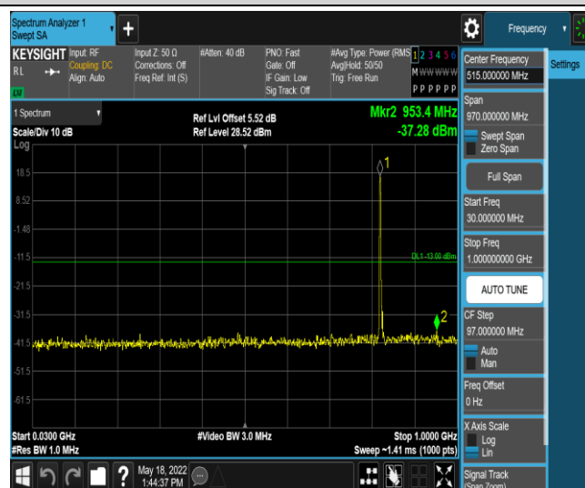
Band5-3MHz-16QAM-20415-1RB#0-Range3:30~1000MHz
