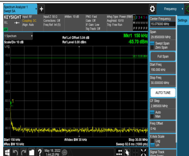
Band5-3MHz-16QAM-20415-1RB#0-Range2:0.15~30MHz
