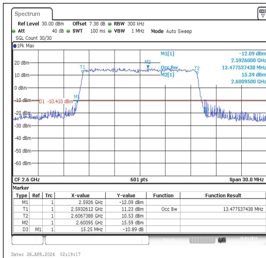
41(2555-2655)-15MHz-QPSK-40690-75RB#0-PA SS
