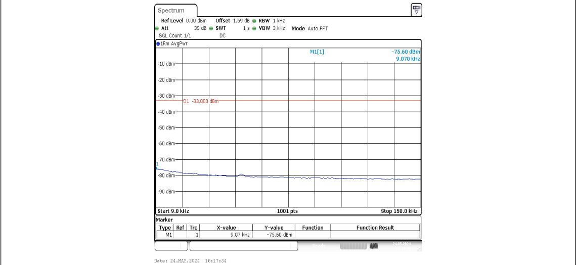
Band5-4182-2-0.009~0.15MHz-PASS
