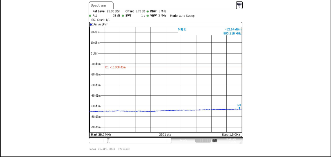
Band2-9262-4-30~1000MHz-PASS
