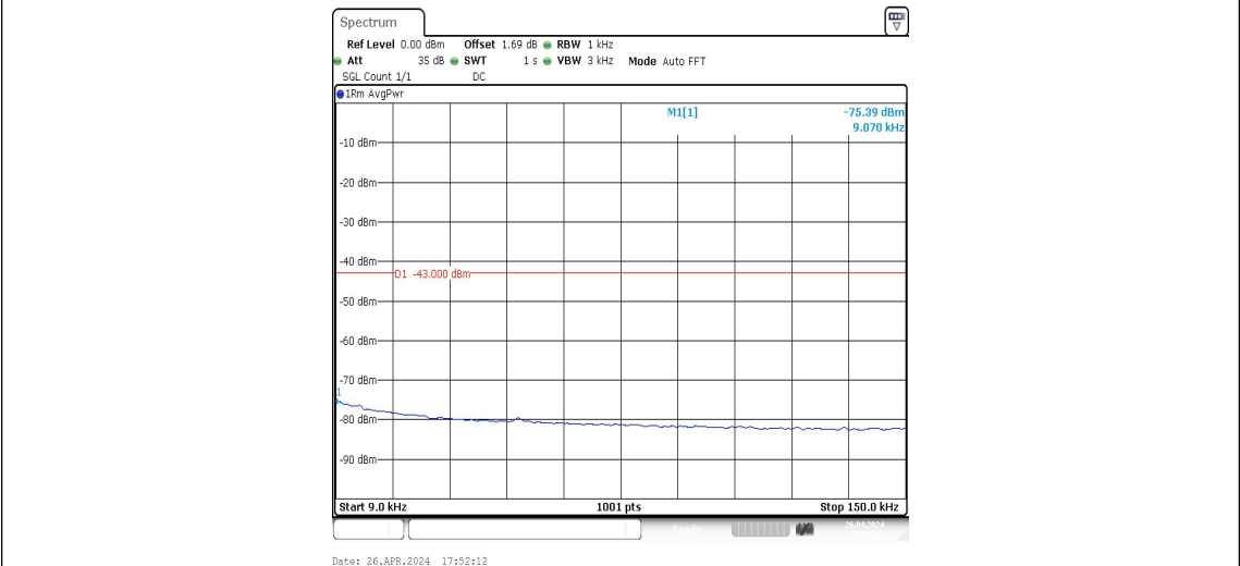
Band2-9538-3-0.009~0.15MHz-PASS
