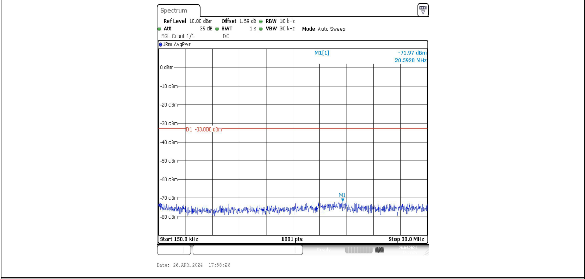
Band2-9400-5-0.15~30MHz-PASS
