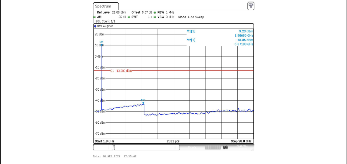
Band2-9538-5-1000~20000MHz-PASS
