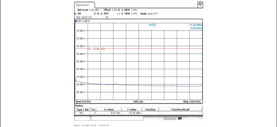
Band5-4182-3-0.009~0.15MHz-PASS
