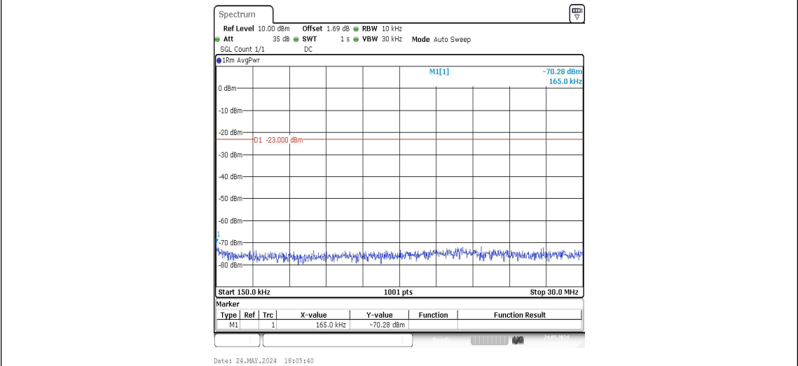
Band5-4182-3-0.15~30MHz-PASS
