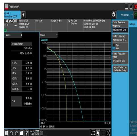
NTNV-N41-PC2-30-20-H-DFT-16QAM-Outter_Full-P PASS
