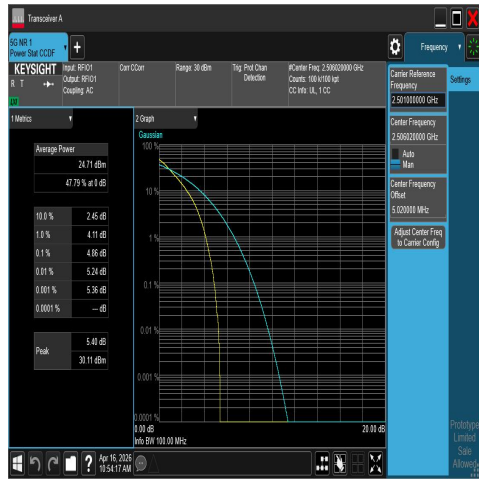
NTNV-N41-PC2-30-20-L-DFT-QPSK-Outter_Full-P ASS
