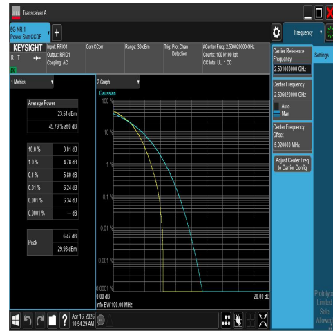
NTNV-N41-PC2-30-20-L-DFT-16QAM-Outter_Full-P PASS
