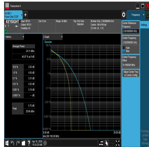
NTNV-N41-PC2-30-20-M-DFT-16QAM-Outter_Full-P PASS
