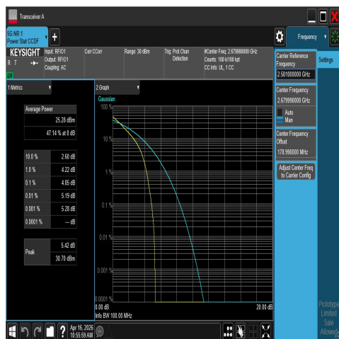
NTNV-N41-PC2-30-20-H-DFT-QPSK-Outter_Full-P ASS
