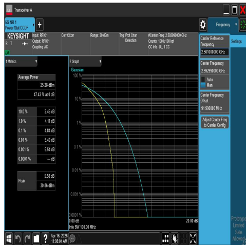
NTNV-N41-PC2-30-70-M-DFT-QPSK-Outter_Full-P ASS
