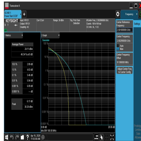
NTNV-N41-PC2-30-50-M-DFT-16QAM-Outter_Full-P PASS
