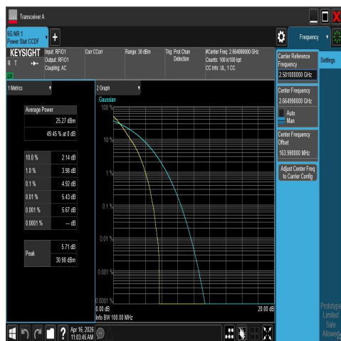
NTNV-N41-PC2-30-50-H-DFT-QPSK-Outter_Full-P ASS
