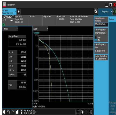
NTNV-N41-PC2-30-40-M-DFT-QPSK-Outter_Full-P ASS
