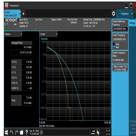
NTNV-N41-PC2-30-100-M-DFT-16QAM-Outer_Ful I-PASS
