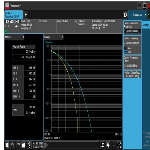
NTNV-N41-PC2-30-70-L-DFT-16QAM-Outter_Full-P PASS
