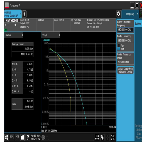
NTNV-N41-PC2-30-50-L-DFT-16QAM-Outter_Full-P PASS
