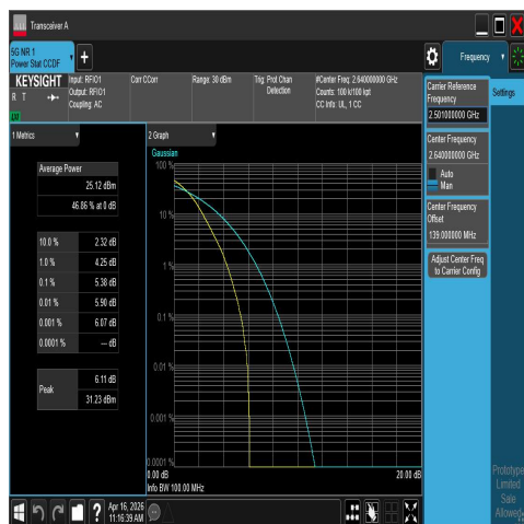
NTNV-N41-PC2-30-100-H-DFT-QPSK-Outer_Full-PASS
