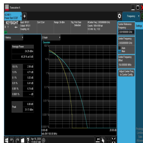
NTNV-N41-PC2-30-70-H-DFT-16QAM-Outter_Full-P PASS
