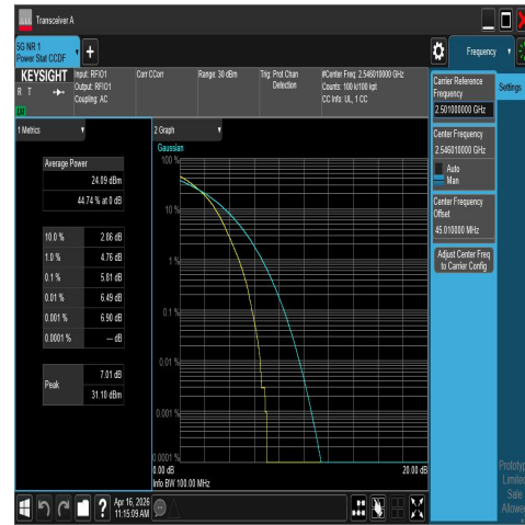
NTNV-N41-PC2-30-100-L-DFT-16QAM-Outer_Full-PASS
