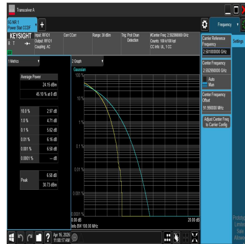
NTNV-N41-PC2-30-70-M-DFT-16QAM-Outter_Full-P PASS
