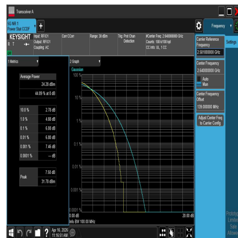
NTNV-N41-PC2-30-100-H-DFT-16QAM-Outer_Ful I-PASS
