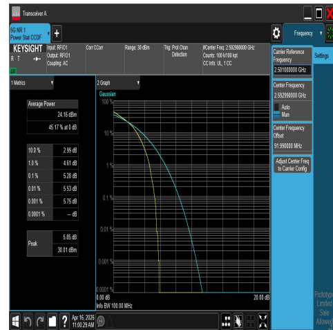
NTNV-N41-PC2-30-40-M-DFT-16QAM-Outter_Full-P PASS
