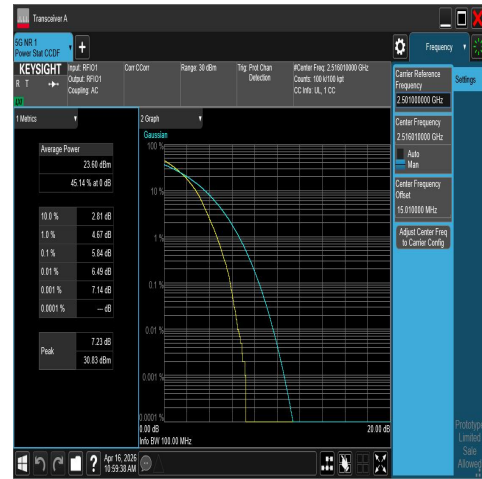
NTNV-N41-PC2-30-40-L-DFT-16QAM-Outter_Full-P PASS
