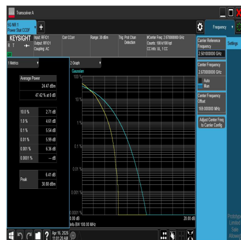
NTNV-N41-PC2-30-40-H-DFT-16QAM-Outter_Full-P PASS
