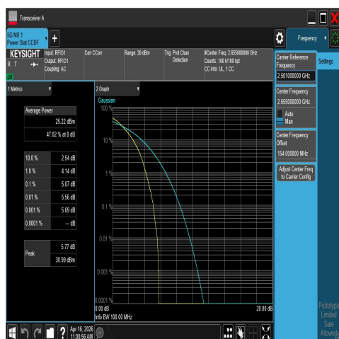
NTNV-N41-PC2-30-70-H-DFT-QPSK-Outter_Full-P ASS
