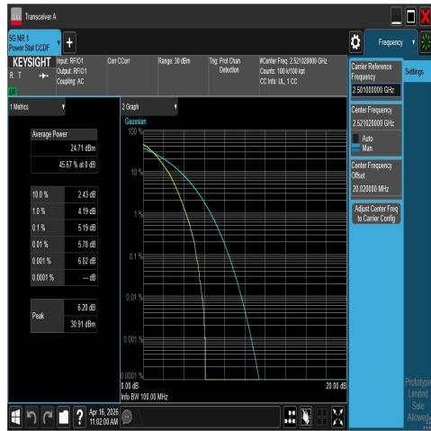
NTNV-N41-PC2-30-50-L-DFT-QPSK-Outter_Full-P ASS
