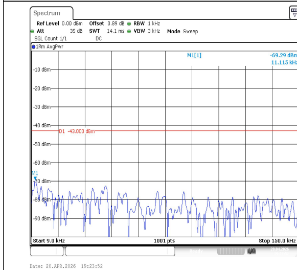
Band2-1.4MHz-QPSK-18900-1RB#0-0.009~0.15-PASS
