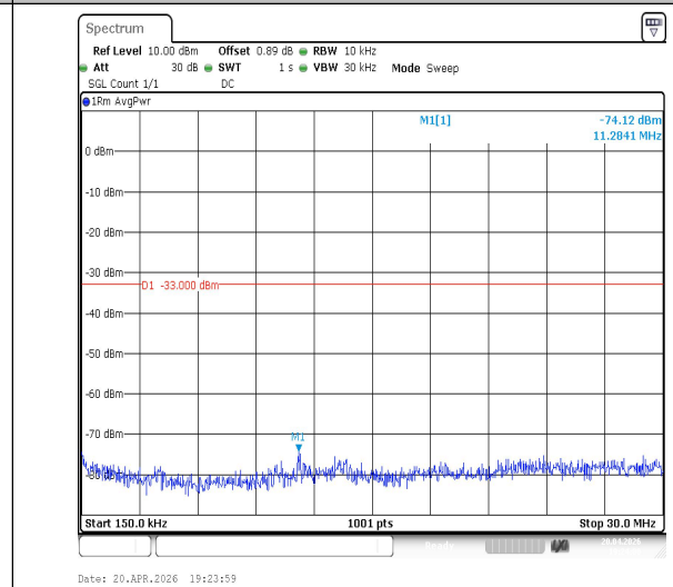
Band2-1.4MHz-QPSK-18900-1RB#0-0.15~30-PASS
