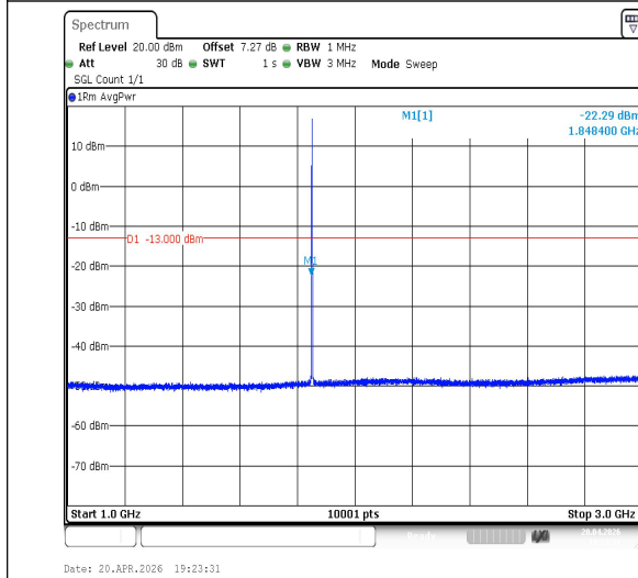
Band2-1.4MHz-16QAM-18607-1RB#0-1000~3000-PASS
