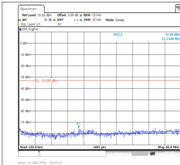
Band2-1.4MHz-16QAM-18607-1RB#0-0.15~30-PASS
