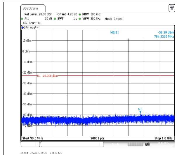
Band2-1.4MHz-16QAM-18607-1RB#0-30~1000-PASS
