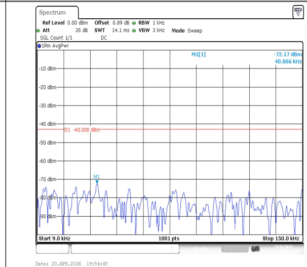
Band2-3MHz-16QAM-18900-1RB#0-0.009~0.15-PASS
