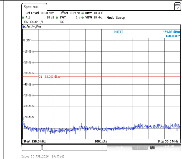
Band2-3MHz-QPSK-19185-1RB#0-0.15~30-PASS
