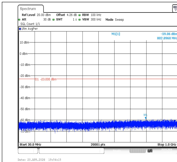
Band2-3MHz-QPSK-18900-1RB#0-30~1000-PASS
