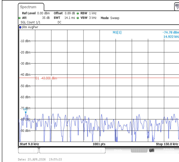
Band2-3MHz-QPSK-19185-1RB#0-0.009~0.15-PASS
