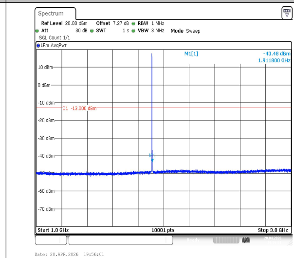
Band2-3MHz-QPSK-19185-1RB#0-1000~3000-PASS
