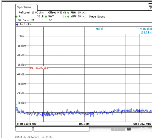
Band2-3MHz-16QAM-18900-1RB#0-0.15~30-PASS
