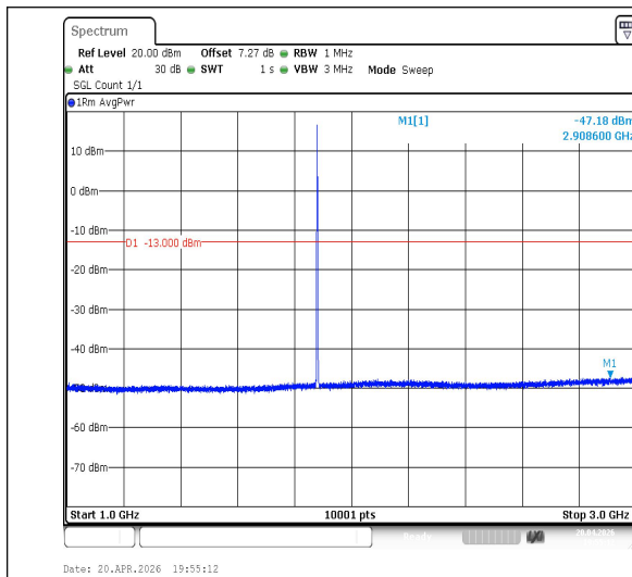
Band2-3MHz-16QAM-18900-1RB#0-1000~3000-PASS
