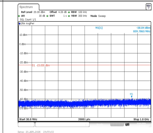
Band2-3MHz-16QAM-18900-1RB#0-30~1000-PASS
