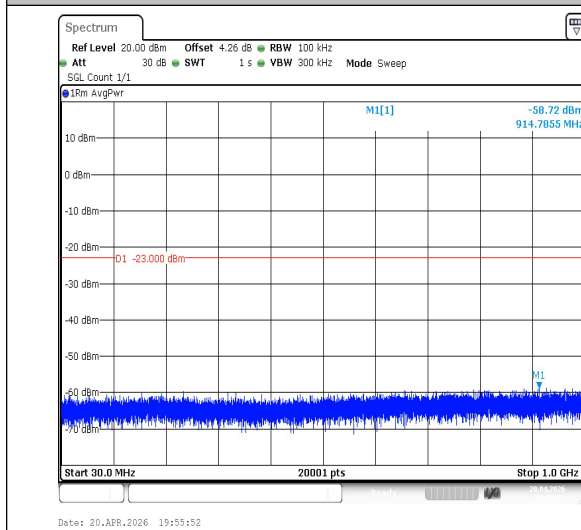
Band2-3MHz-QPSK-19185-1RB#0-30~1000-PASS
