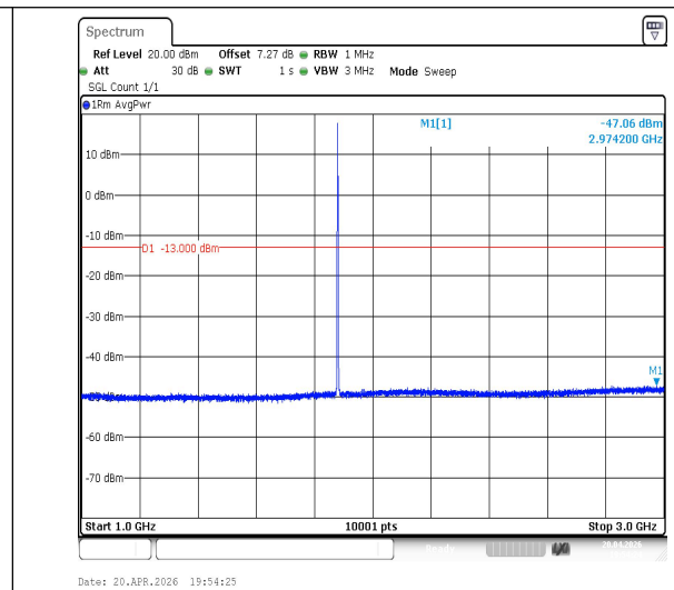
Band2-3MHz-QPSK-18900-1RB#0-1000~3000-PASS
