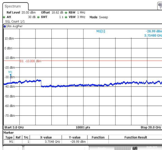
Band2-10MHz-QPSK-19150-1RB#0-3000~20000-PASS
