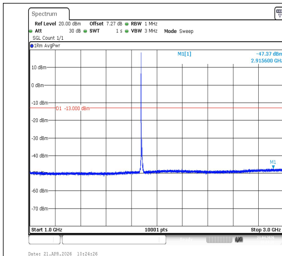
Band2-10MHz-16QAM-18900-1RB#0-1000~3000-PASS
