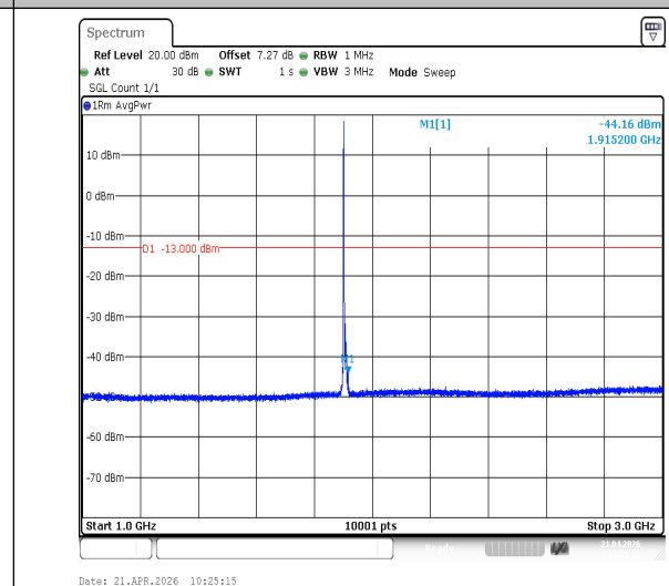
Band2-10MHz-QPSK-19150-1RB#0-1000~3000-PASS
