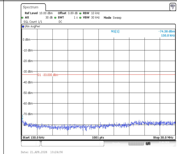
Band2-10MHz-QPSK-19150-1RB#0-0.15~30-PASS
