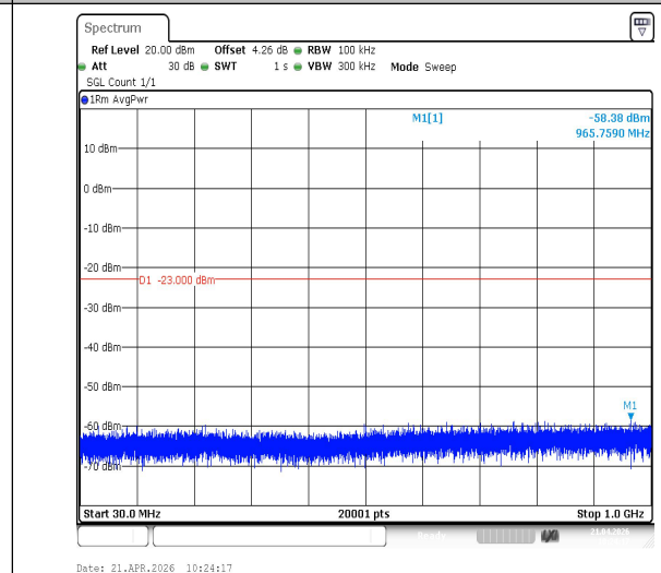
Band2-10MHz-16QAM-18900-1RB#0-30~1000-PASS
