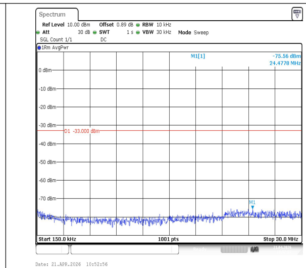
Band2-15MHz-QPSK-18675-1RB#0-0.15~30-PASS
