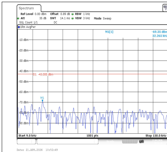
Band2-15MHz-QPSK-18675-1RB#0-0.009~0.15-PASS
