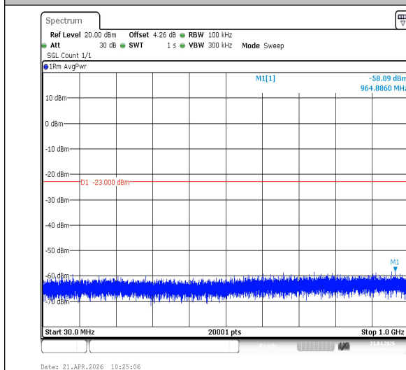
Band2-10MHz-QPSK-19150-1RB#0-30~1000-PASS
