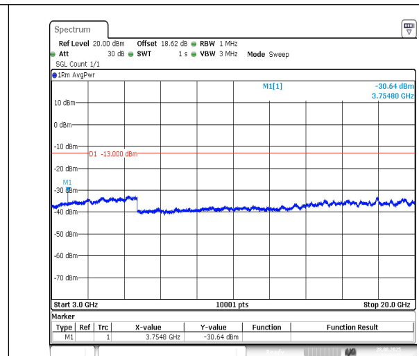
Band2-10MHz-16QAM-18900-1RB#0-3000~20000-PASS
