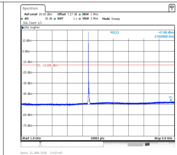
Band2-10MHz-QPSK-18900-1RB#0-1000~3000-PASS
