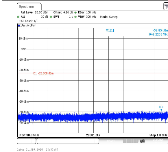
Band2-15MHz-QPSK-18675-1RB#0-30~1000-PASS
