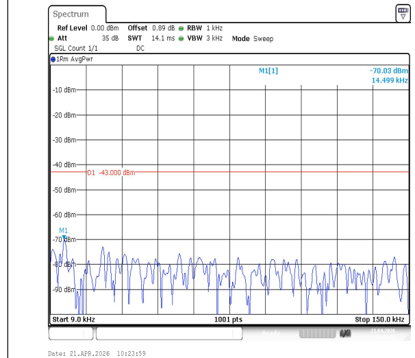
Band2-10MHz-16QAM-18900-1RB#0-0.009~0.15-PASS
