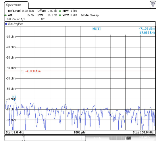
Band2-10MHz-16QAM-19150-1RB#0-0.009~0.15-PASS
