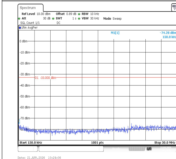
Band2-10MHz-16QAM-18900-1RB#0-0.15~30-PASS
