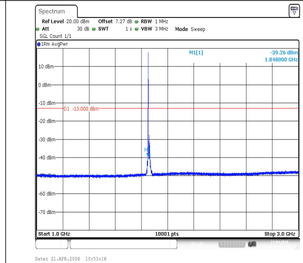
Band2-15MHz-QPSK-18675-1RB#0-1000~3000-PASS
