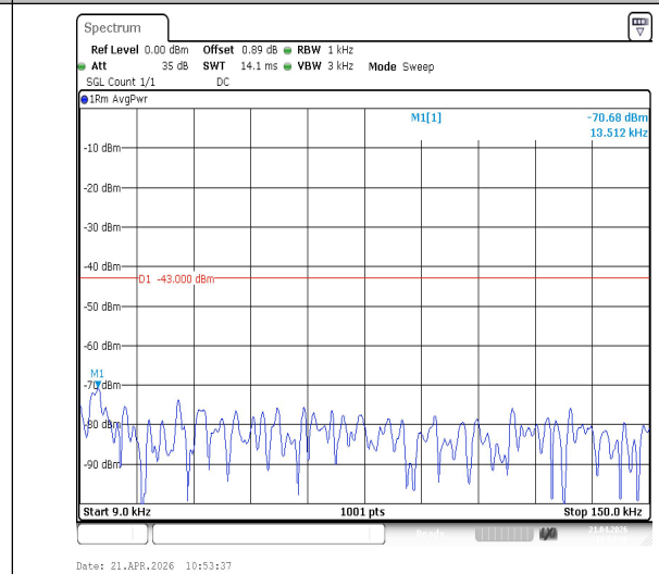
Band2-15MHz-16QAM-18675-1RB#0-0.009~0.15-PASS
