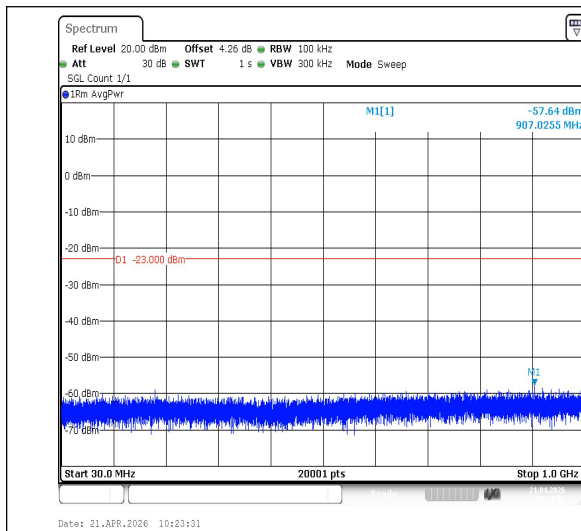
Band2-10MHz-QPSK-18900-1RB#0-30~1000-PASS
