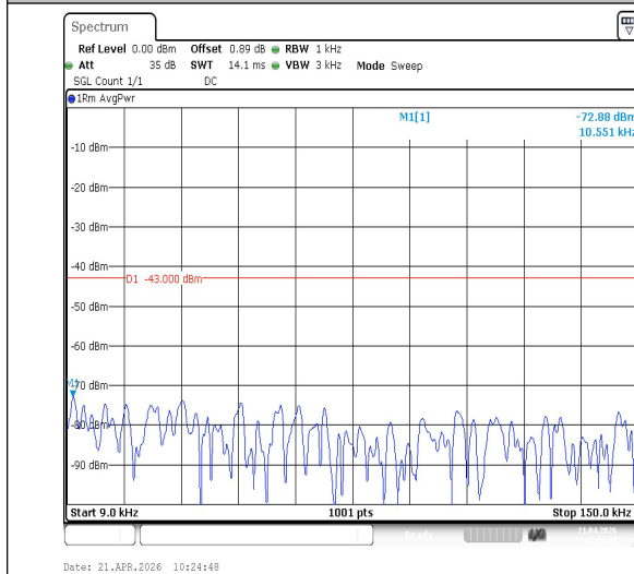
Band2-10MHz-QPSK-19150-1RB#0-0.009~0.15-PASS
