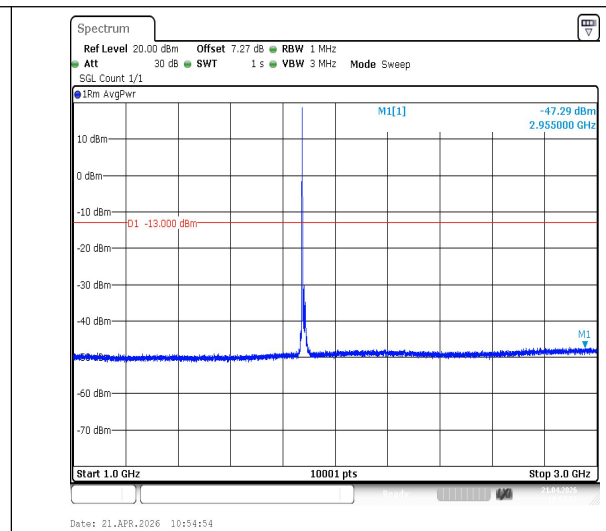
Band2-15MHz-QPSK-18900-1RB#0-1000~3000-PASS
