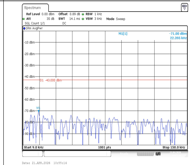
Band2-15MHz-16QAM-18900-1RB#0-0.009~0.15-PASS
