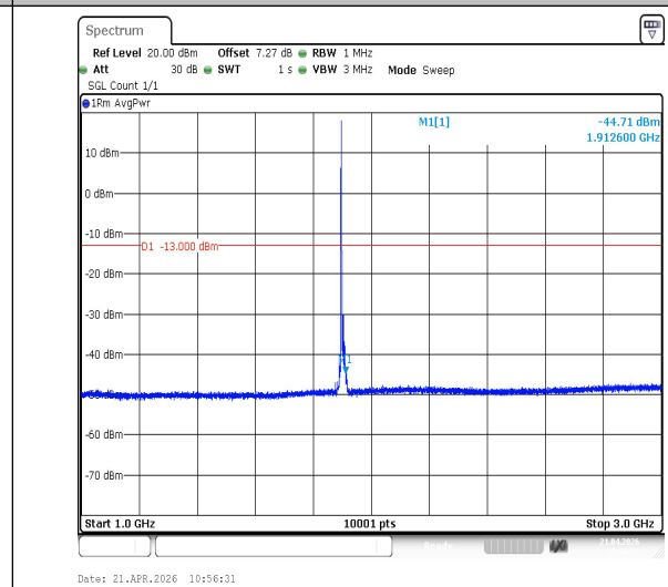
Band2-15MHz-QPSK-19125-1RB#0-1000~3000-PASS
