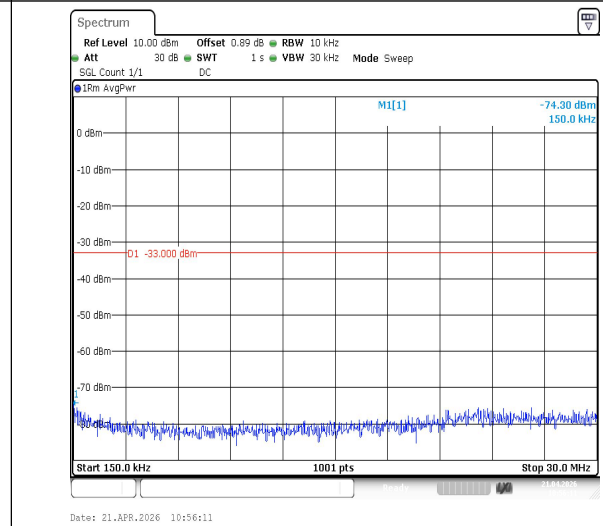
Band2-15MHz-QPSK-19125-1RB#0-0.15~30-PASS
