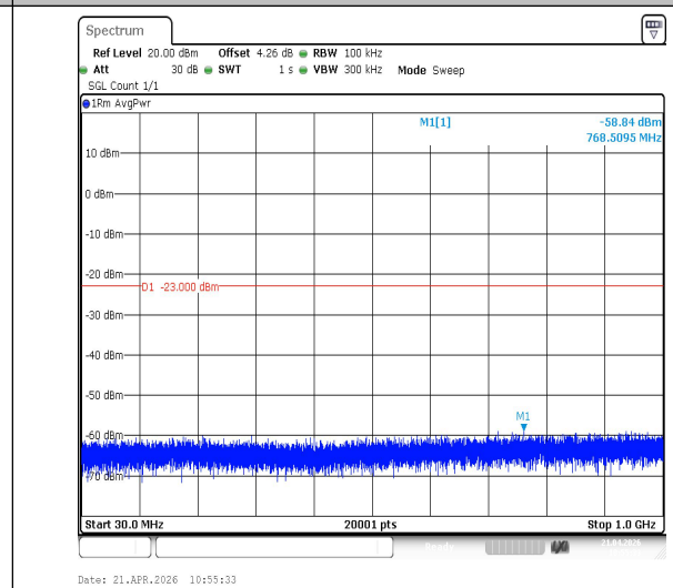
Band2-15MHz-16QAM-18900-1RB#0-30~1000-PASS
