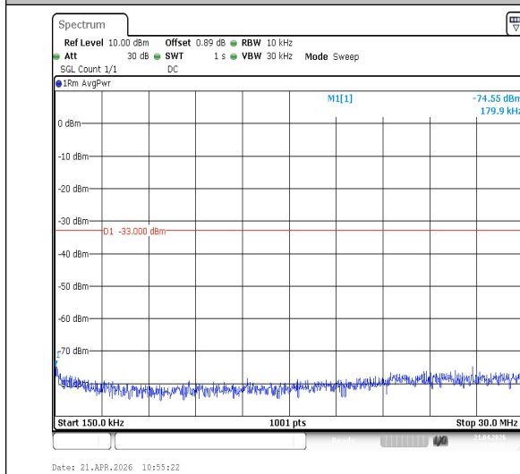
Band2-15MHz-16QAM-18900-1RB#0-0.15~30-PASS
