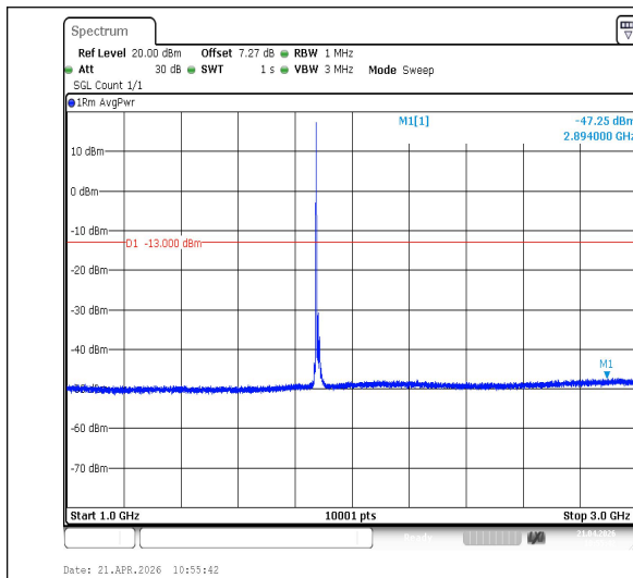
Band2-15MHz-16QAM-18900-1RB#0-1000~3000-PASS
