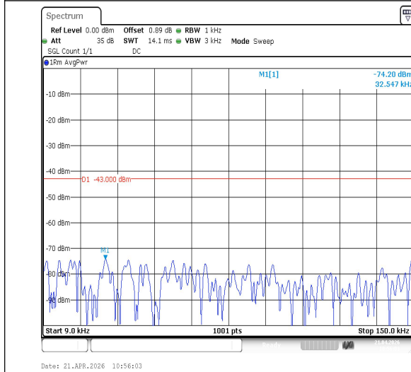
Band2-15MHz-QPSK-19125-1RB#0-0.009~0.15-PASS
