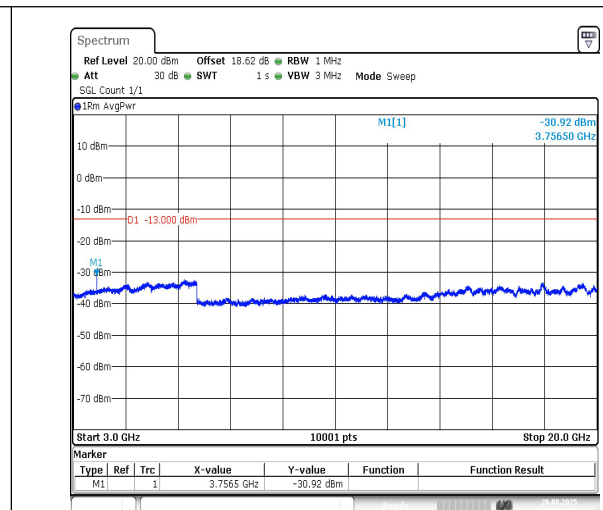
Band2-15MHz-16QAM-18900-1RB#0-3000~20000-PASS
