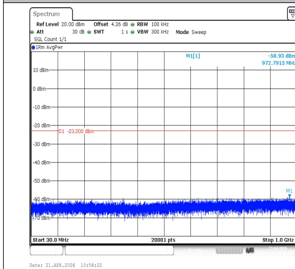
Band2-15MHz-QPSK-19125-1RB#0-30~1000-PASS
