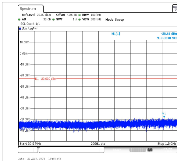
Band2-15MHz-QPSK-18900-1RB#0-30~1000-PASS
