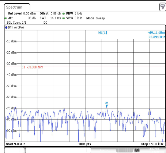
26(824-849)-10MHz-16QAM-26915-1RB#0-1000 ~3000-PASS
