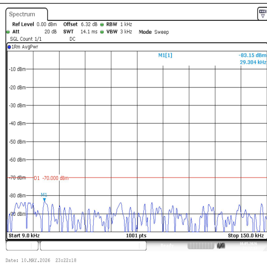
Band30-5MHz-16QAM-27685-1RB#0-0.009~0.15- PASS
