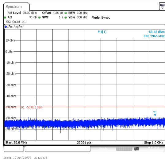
Band30-5MHz-16QAM-27685-1RB#0-30~1000-PA SS
