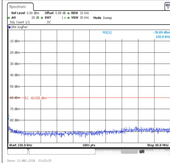
Band30-5MHz-16QAM-27685-1RB#0-0.15~30-PA SS
