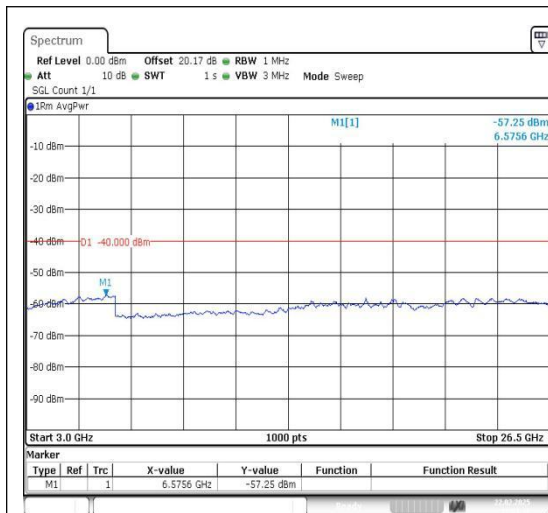
Band30-5MHz-QPSK-27685-1RB#0-3000~26500 -PASS
