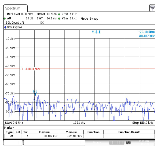
Band4-3MHz-16QAM-20385-1RB#0-0.009~0.15-P ASS
