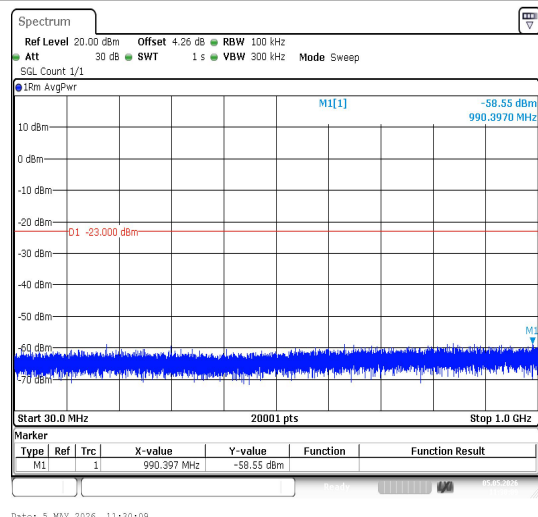
Band4-3MHz-16QAM-20385-1RB#0-30~1000-PAS S
