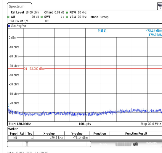
Band4-3MHz-16QAM-20385-1RB#0-0.15~30-PA SS
