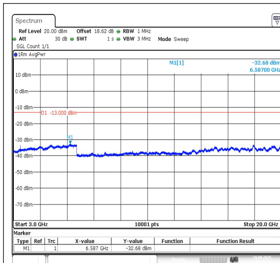
Band4-3MHz-QPSK-20385-1RB#0-3000~20000- PASS
