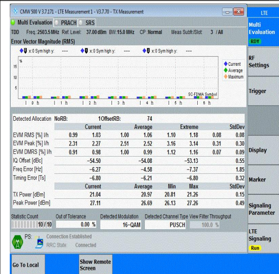
Band41-15MHz-16QAM-39725-1RB#74-PASS
