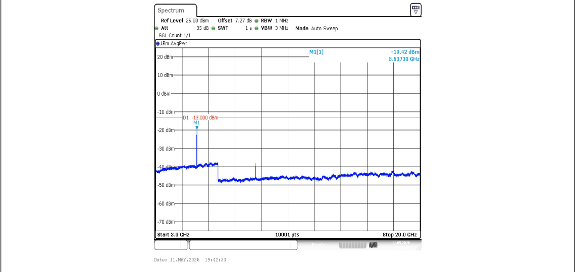
Band2-9400-5-3000~20000MHz-PASS
