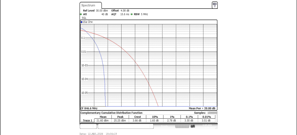
Band5-4233-PASS
