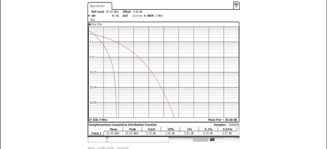
Band5-4182-PASS
