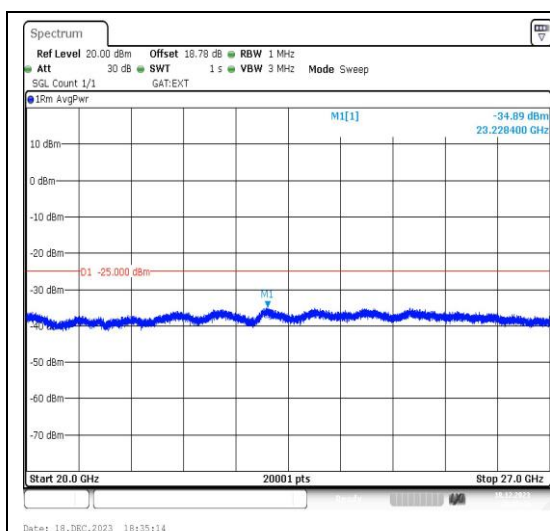
Band41_5MHz_QPSK_40265_1RB#0_20000~27000 000_20000~27000
