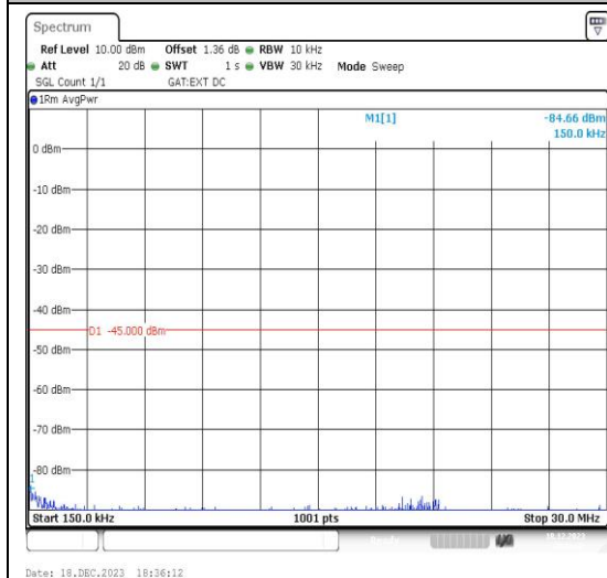
Band41_5MHz_16QAM_40265_1RB#0_0.15~30 _0.15~30
