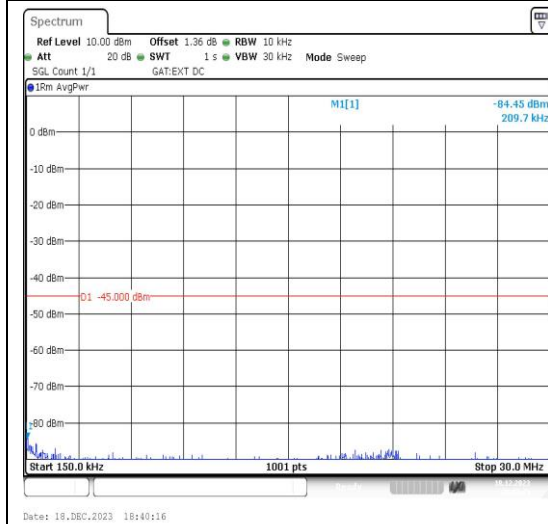
Band41_5MHz_16QAM_40690_1RB#0_0.15~30 _0.15~30
