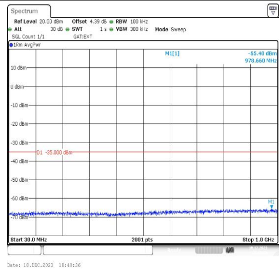
Band41_5MHz_16QAM_40690_1RB#0_30~1000_ 30~1000
