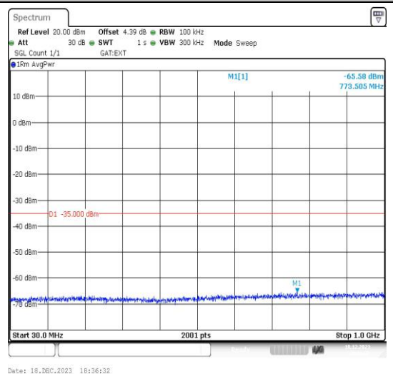
Band41_5MHz_16QAM_40265_1RB#0_30~1000 30~1000
