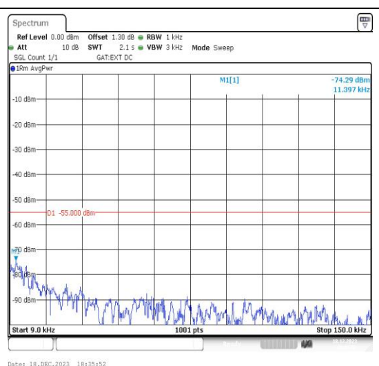
Band41_5MHz_16QAM_40265_1RB#0_0.009~0.15 5_0.009~0.15
