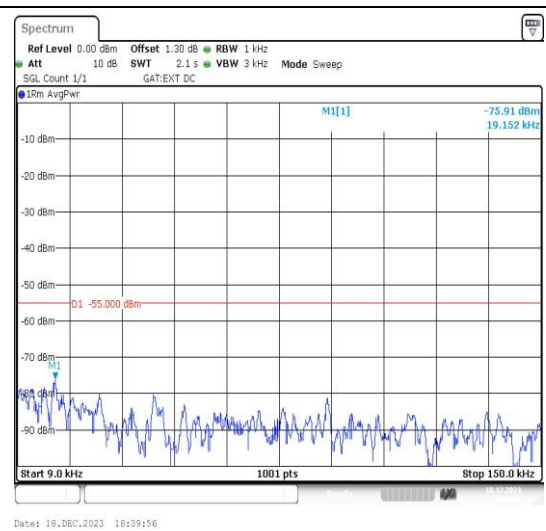
Band41_5MHz_16QAM_40690_1RB#0_0.009~0.15 5_0.009~0.15
