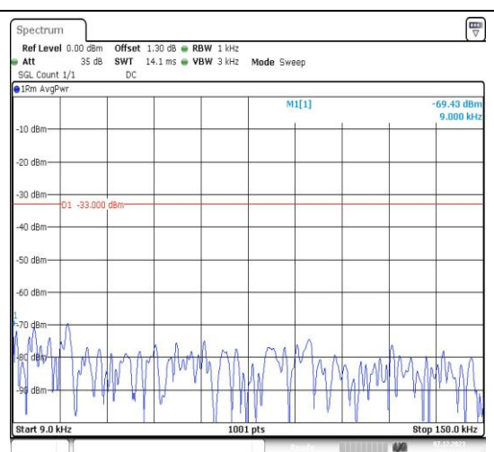
Band5_1.4MHz_16QAM_20525_1RB#0_0.009~0.15_0.009~0.15
