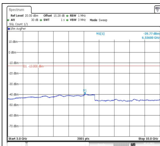
Band5_1.4MHz_QPSK_20525_1RB#0_3000~10000_3000~10000
