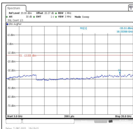
Band66_3MHz_QPSK_132322_1RB#0_3000~20000_3000~20000
