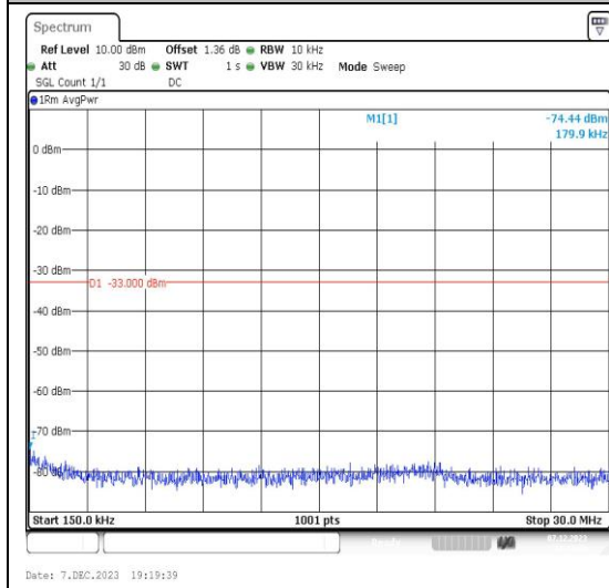
Band66_3MHz_16QAM_132322_1RB#0_0.15~30_0.15~30
