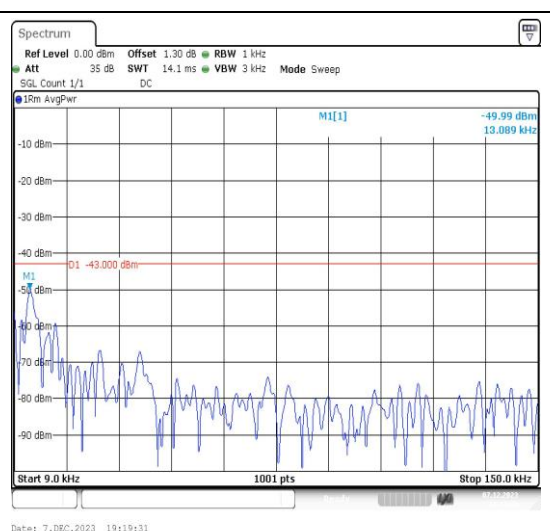
Band66_3MHz_16QAM_132322_1RB#0_0.009~0.15_0.009~0.15
