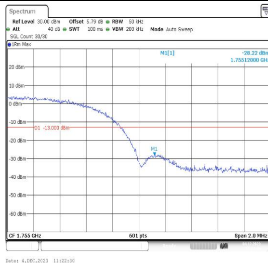
Band4-1513-2-PASS
