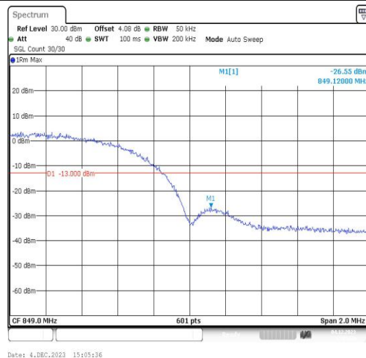
Band5-4233-4-PASS
