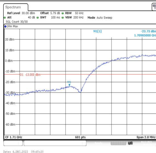
Band4-1312-3-PASS
