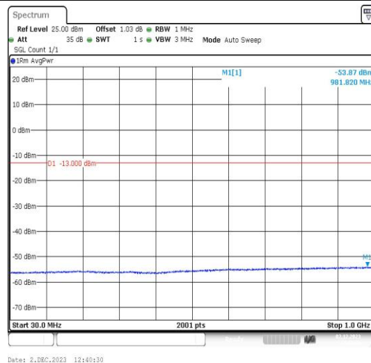
Band2-9400-30~1000MHz-PASS
