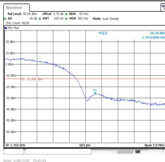
Band4-1513-3-PASS
