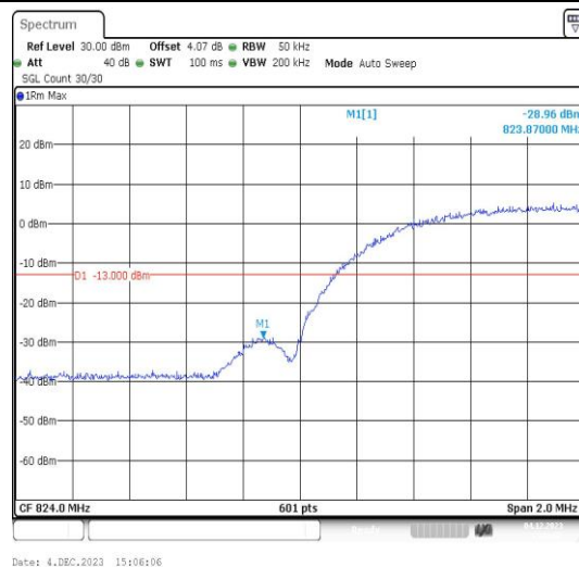
Band5-4132-5-PASS
