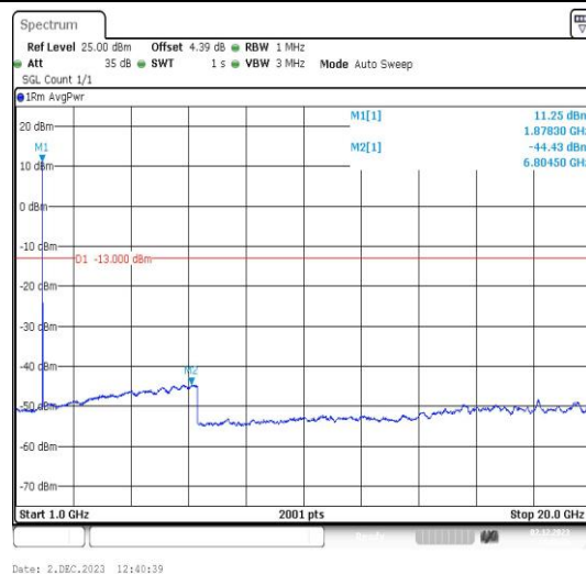
Band2-9400-1000~20000MHz-PASS
