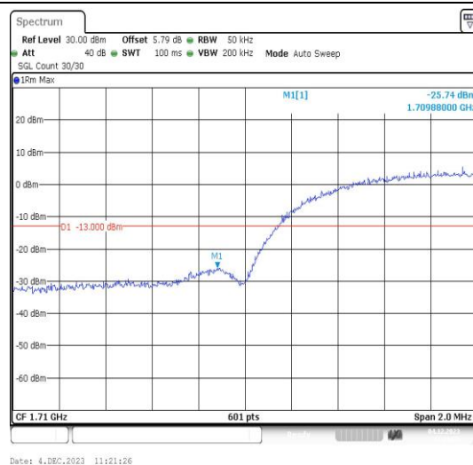
Band4-1312-2-PASS
