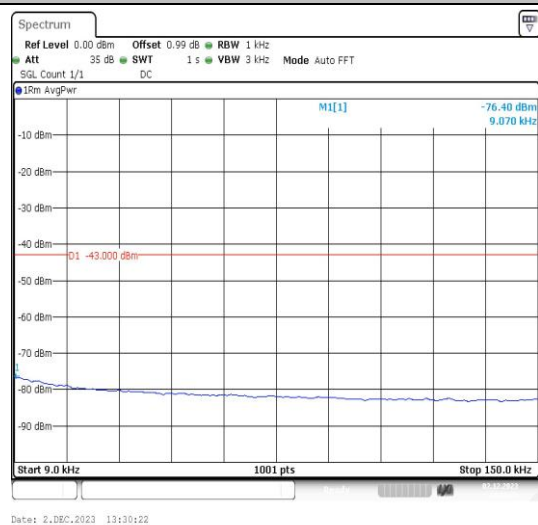
Band2-9538-1-0.009~0.15MHz-PASS
