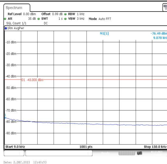
Band2-9538-0.009~0.15MHz-PASS
