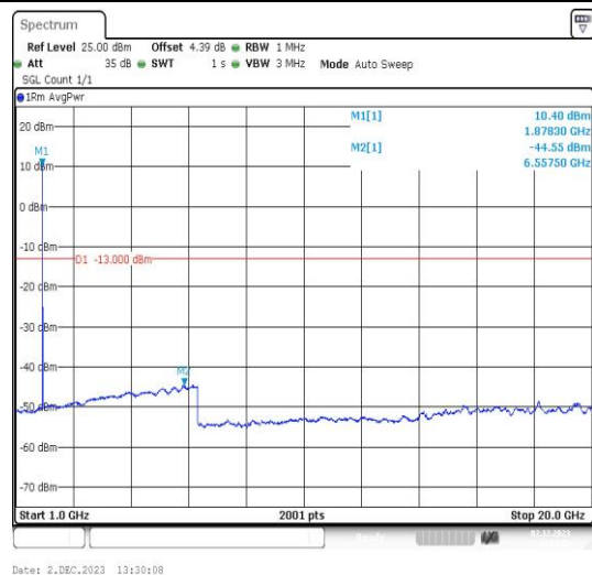
Band2-9400-1-1000~20000MHz-PASS
