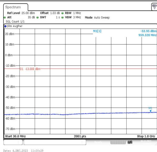
Band4-1413-1-30~1000MHz-PASS
