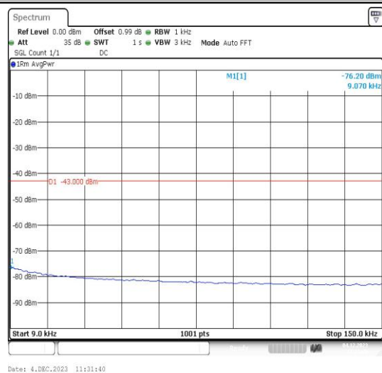
Band4-1513-1-0.009~0.15MHz-PASS
