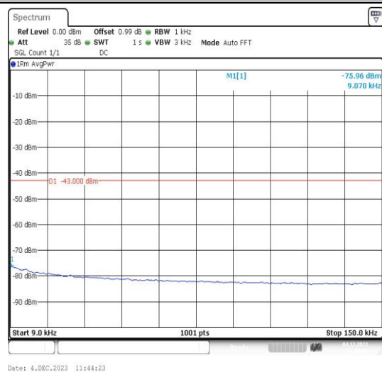
Band4-1513-4-0.009~0.15MHz-PASS
