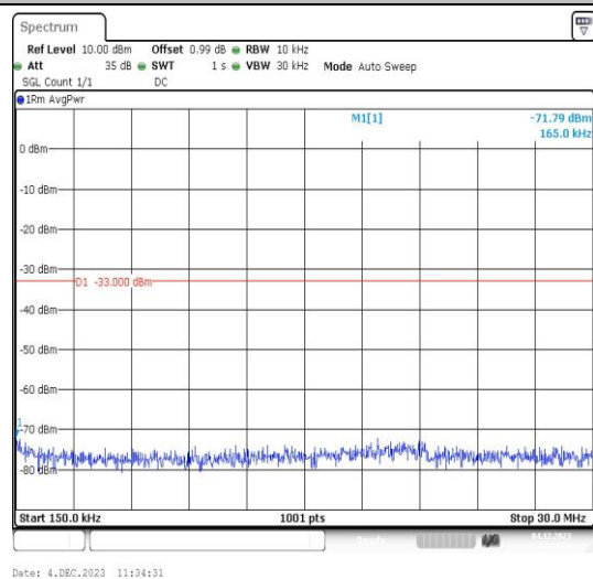
Band4-1413-2-0.15~30MHz-PASS
