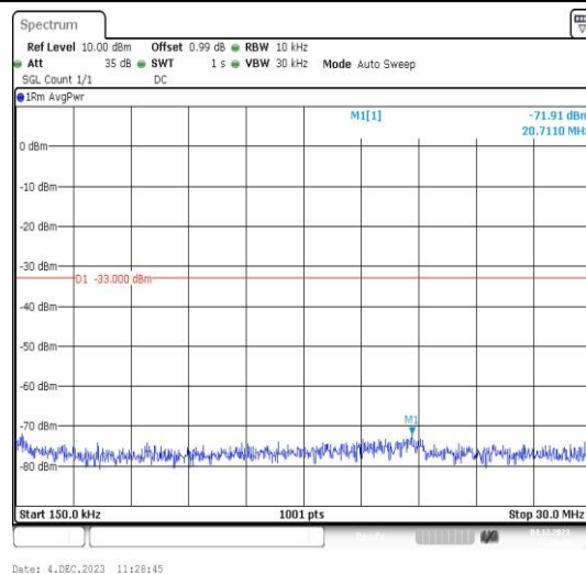
Band4-1312-1-0.15~30MHz-PASS
