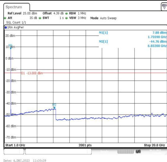
Band4-1413-1-1000~20000MHz-PASS
