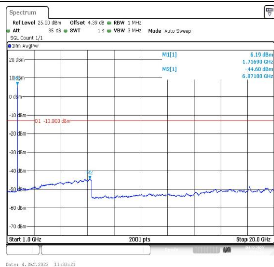
Band4-1312-2-1000~20000MHz-PASS
