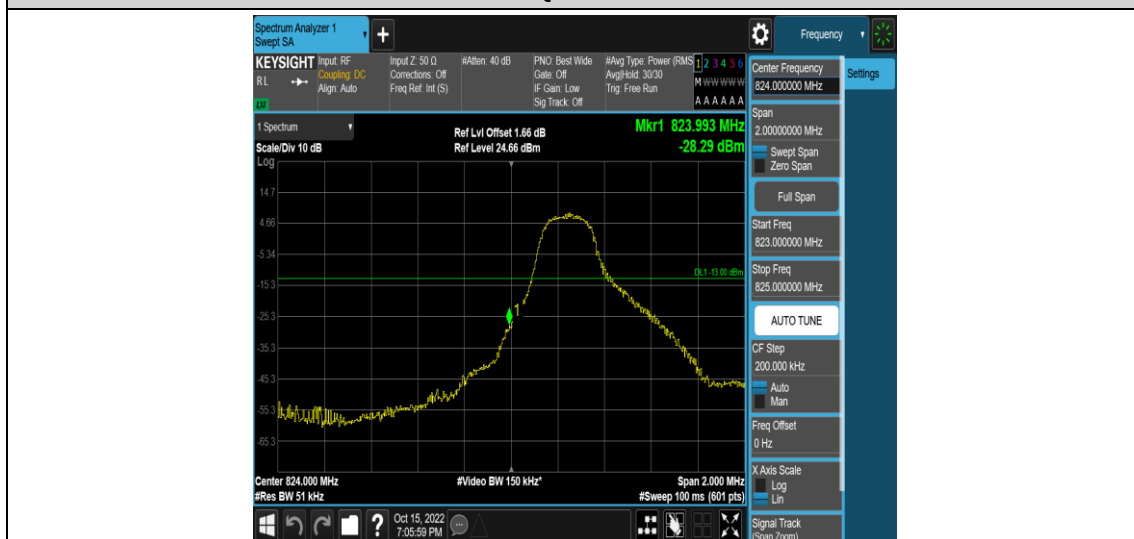
Band5-3MHz-QPSK-20415-1RB#14
