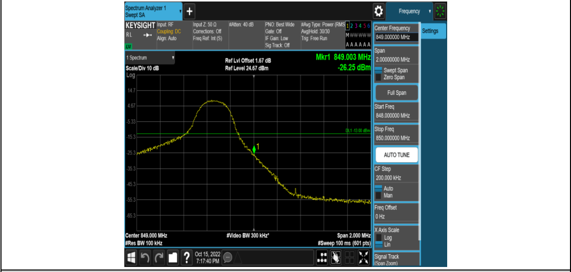
Band5-5MHz-16QAM-20625-25RB#0
