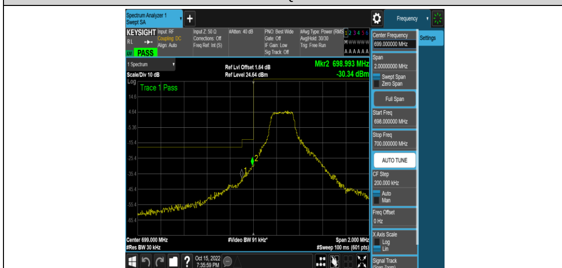
Band12-1.4MHz-16QAM-23017-1RB#5
