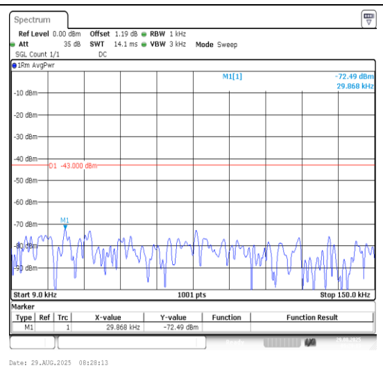
Band66-1.4MHz-16QAM-131979-1RB#0-0.009~0. 15-PASS
