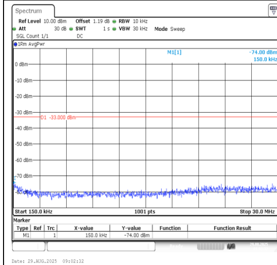
Band66-3MHz-16QAM-131987-1RB#0-0.15~30-P ASS
