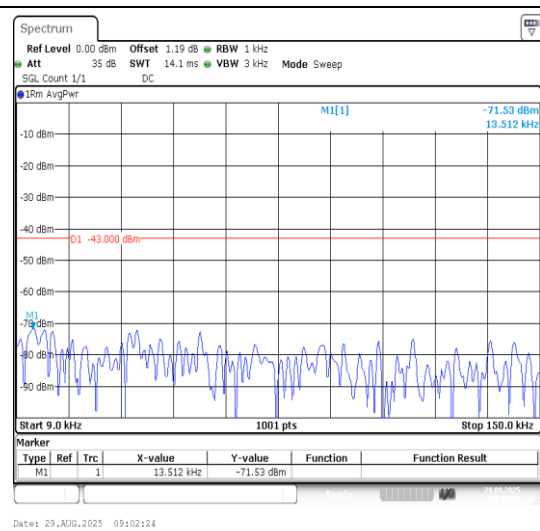
Band66-3MHz-16QAM-131987-1RB#0-0.009~0.15 -PASS
