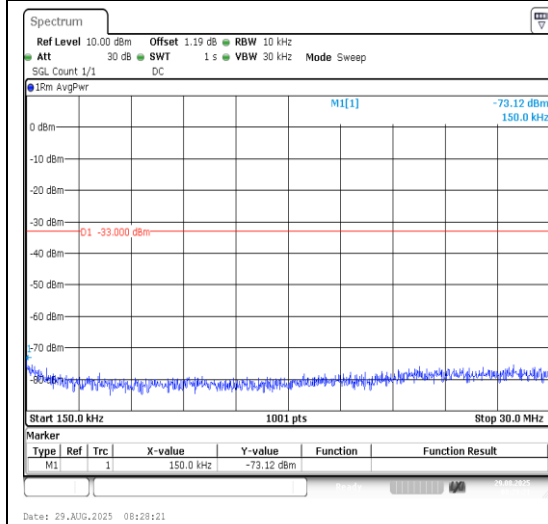
Band66-1.4MHz-16QAM-131979-1RB#0-0.15~30 -PASS
