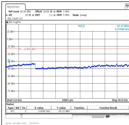
Band66-1.4MHz-QPSK-131979-1RB#0-3000~200 00-PASS
