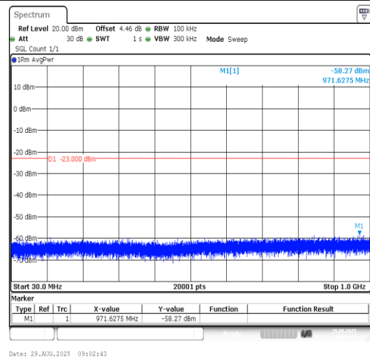
Band66-3MHz-16QAM-131987-1RB#0-30~1000-P ASS
