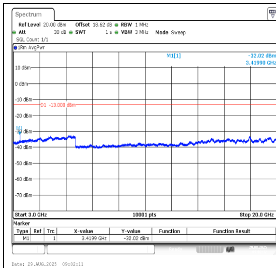
Band66-3MHz-QPSK-131987-1RB#0-3000~2000 0-PASS
