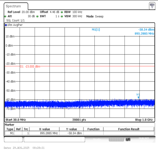
Band66-1.4MHz-16QAM-131979-1RB#0-30~1000- PASS
