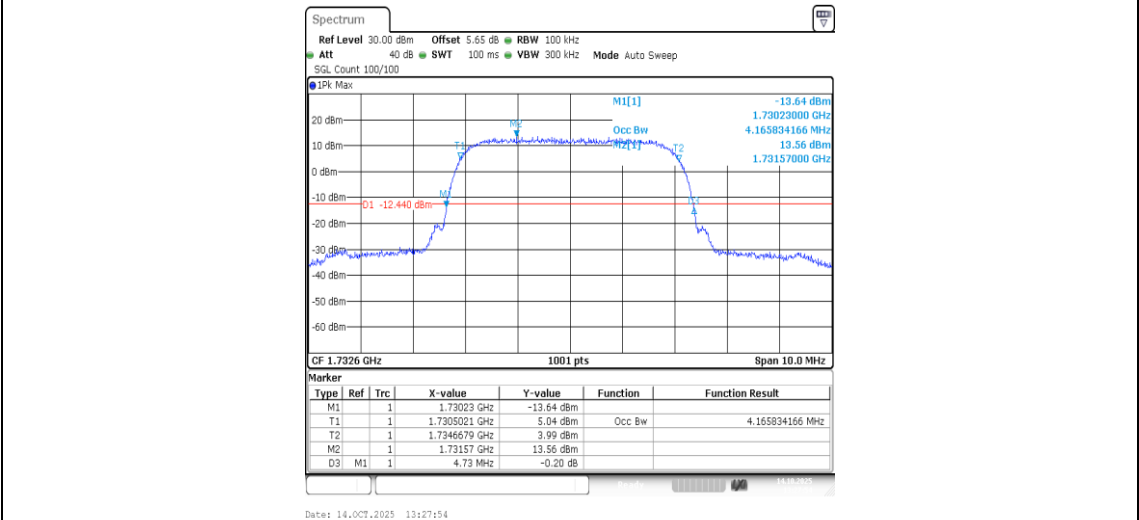
Band4-1413-1-PASS
