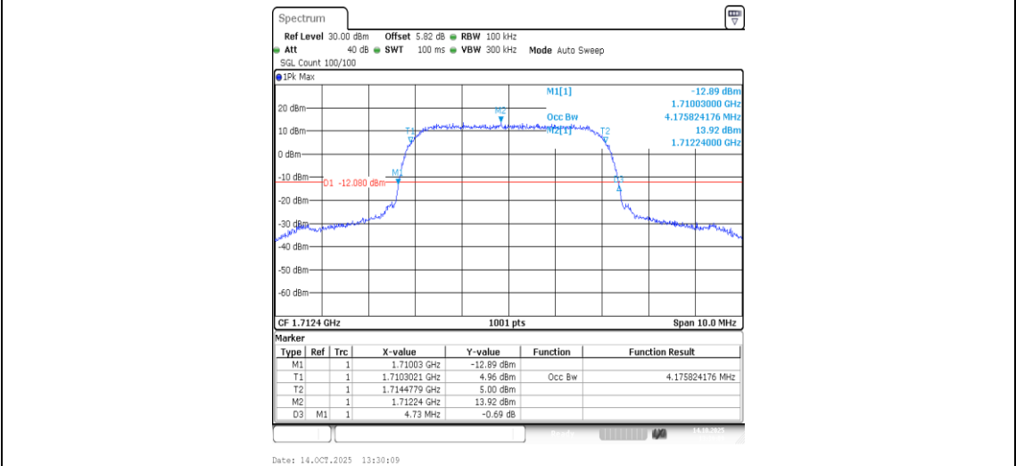
Band4-1312-2-PASS
