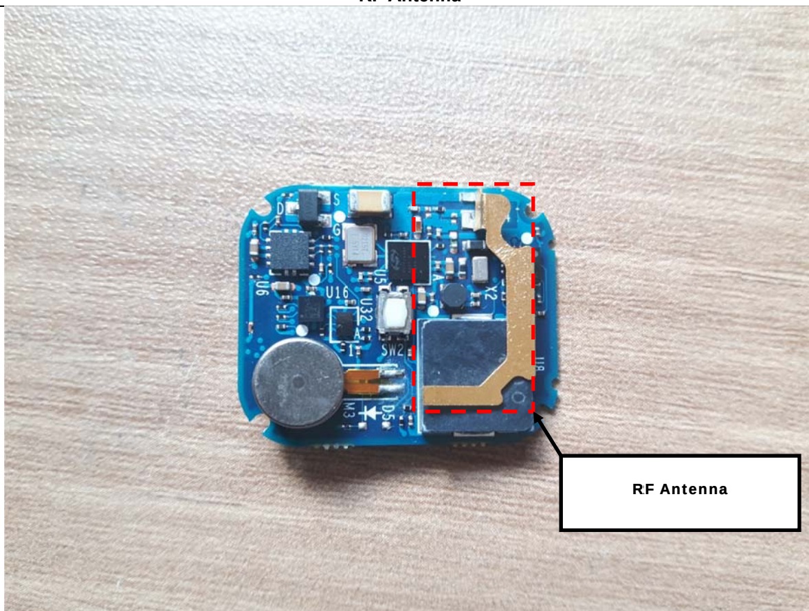
RF Antenna
