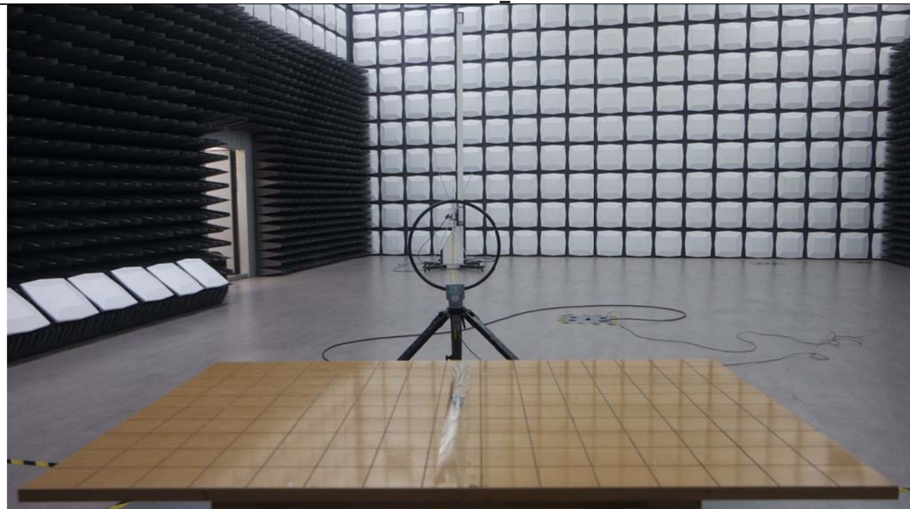
9 kHz – 30 MHz_Rear
