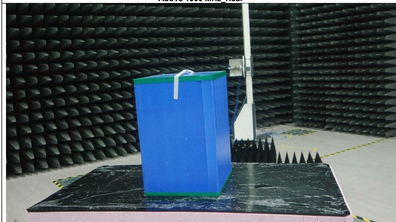
Above 1000 MHz_Rear
