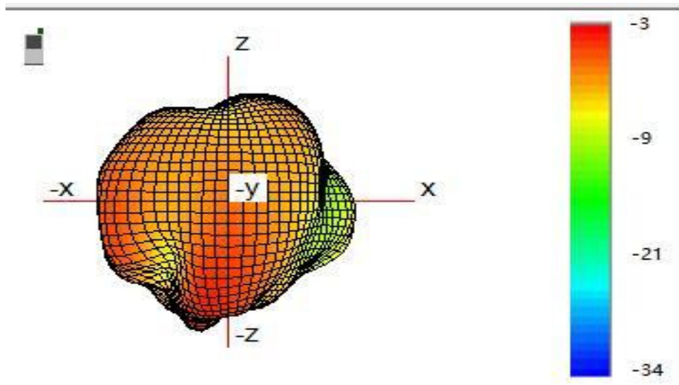
3D Radiation Pattern at 2.45 GHz(unit:dBi):
