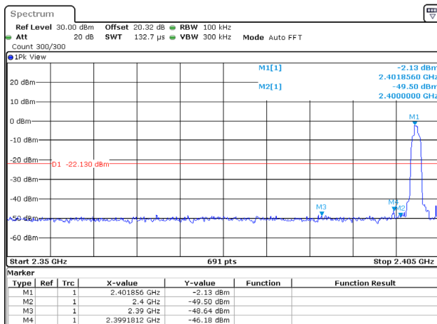
2DH1_Ant1_Low_2402
