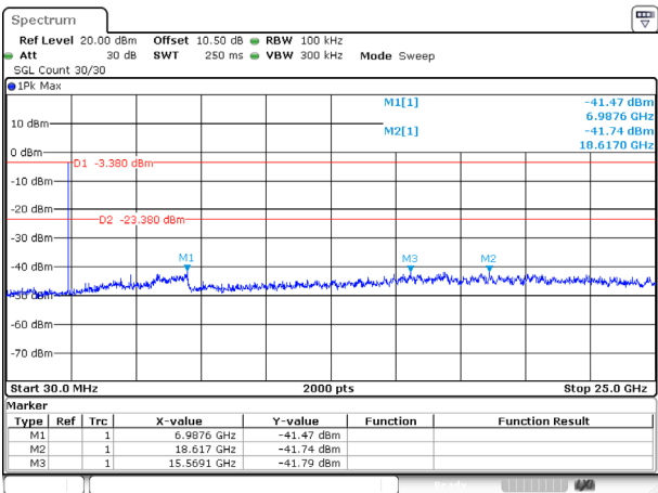
2DH1_Low
