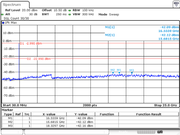
DH1_Middle
