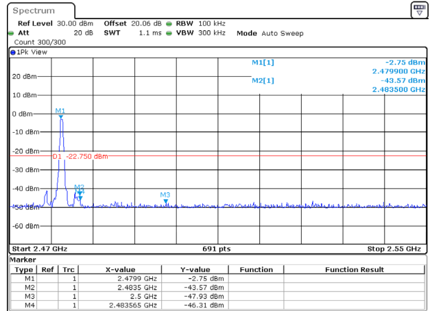
DH1_Ant1_High_2480
