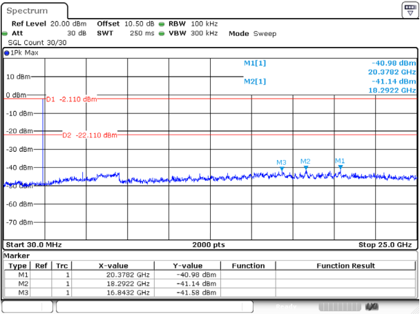
DH1_Low
