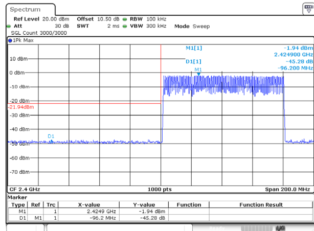
DH1_Hopping_Lower
