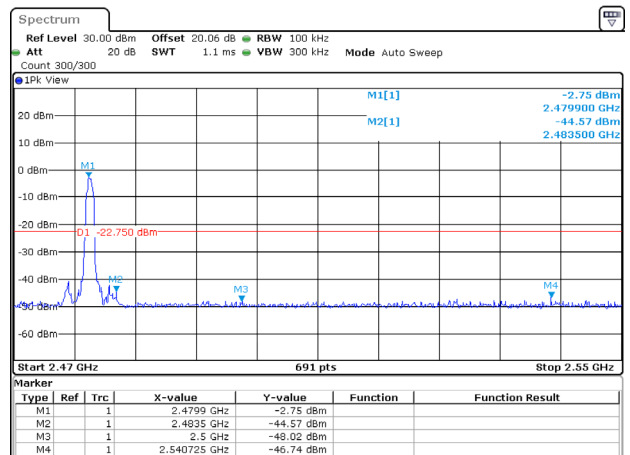
2DH1_Ant1_High_2480
