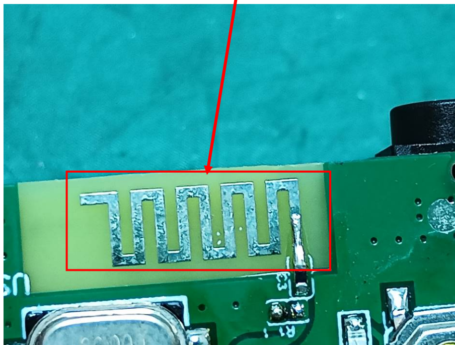
ANT-Bluetooth&BLE
