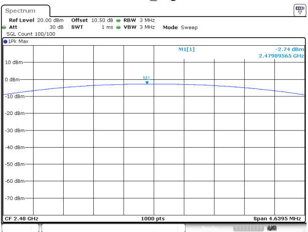
DH5_High
