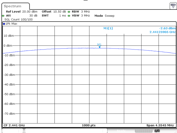
DH5_Middle
