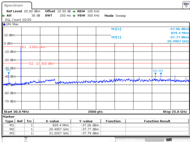
DH1_Low
