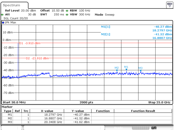
DH5_Low
