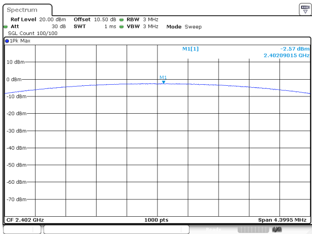
DH1_Low
