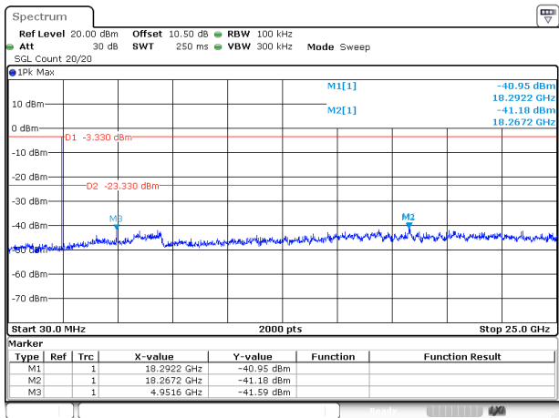
DH1_High
