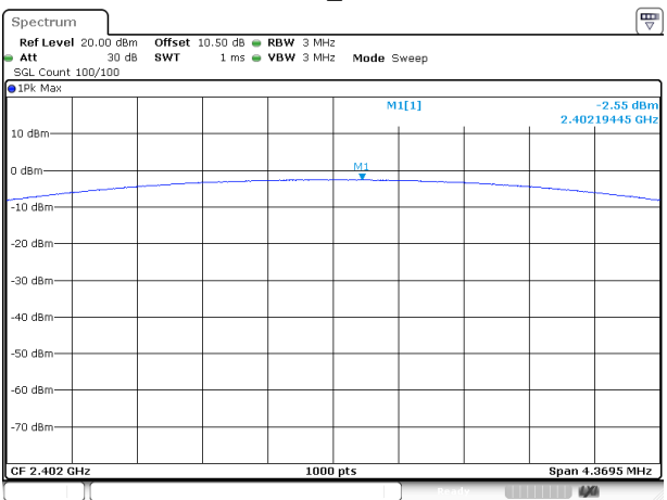
DH5_Low
