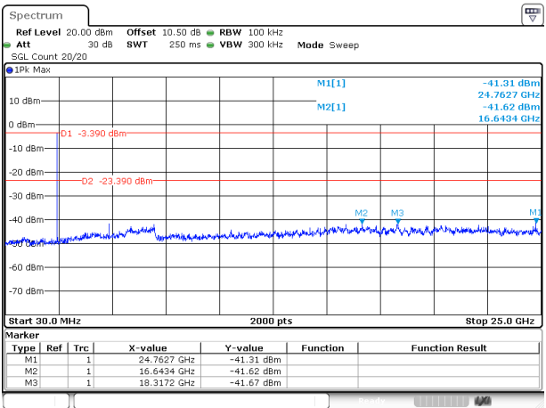
DH1_Middle
