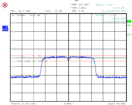
802.11n40_2437MHz
