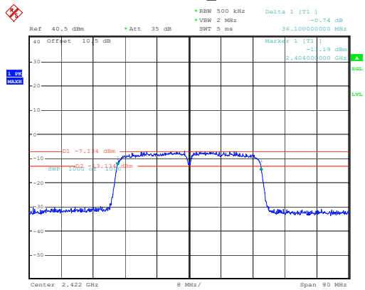
802.11n40_2422MHz
