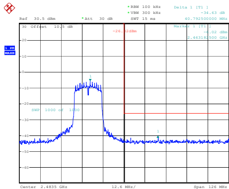
802.11g_2462MHz
