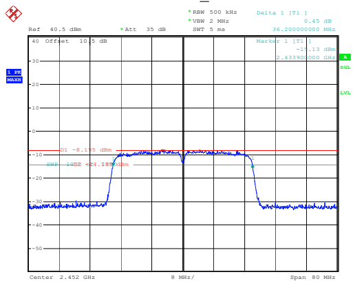
802.11n40_2452MHz
