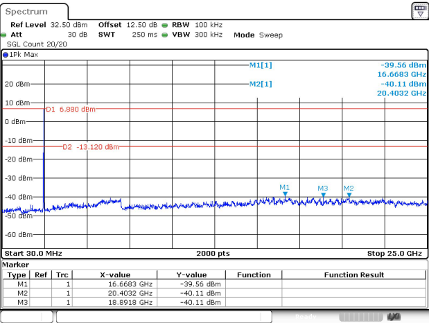
802.11g_2462MHz
