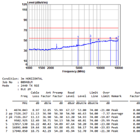
BLE_2M_TX_CH_19_Horizontal
