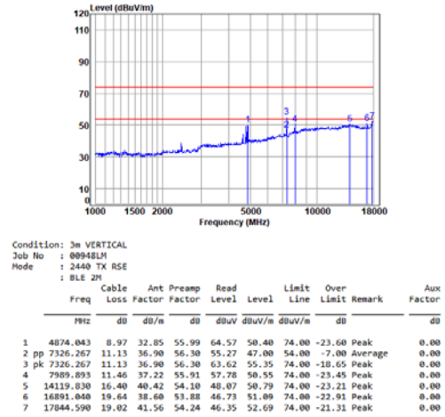
BLE_2M_TX_CH_19_Vertical
