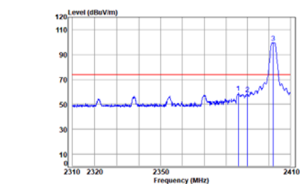
BLE_2M_TX_CH_00_Horizontal-Peak
