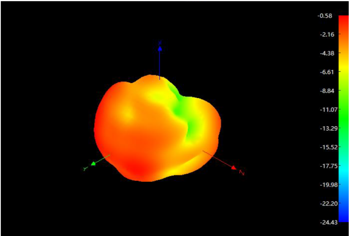
Antenna gain diagram
