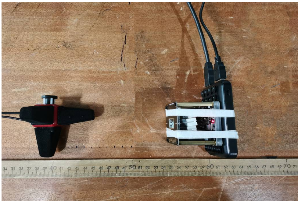
Position E (Distance 20cm)
