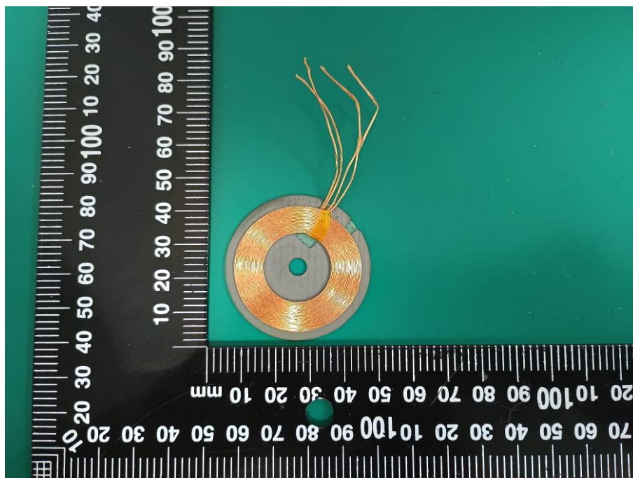
Coil ANT
