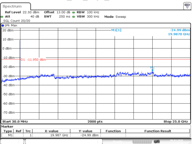
BLE_2M_High_Channel
