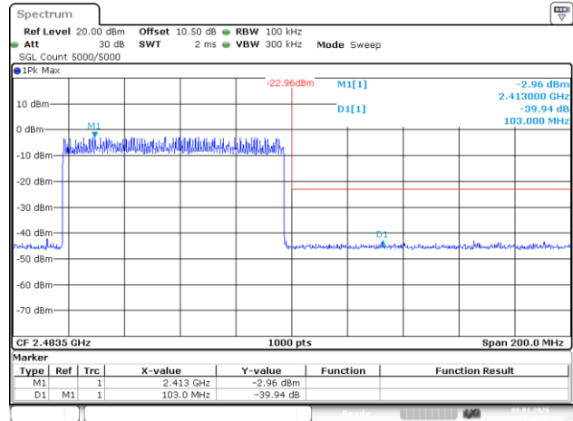
2DH5_Hopping_Upper
