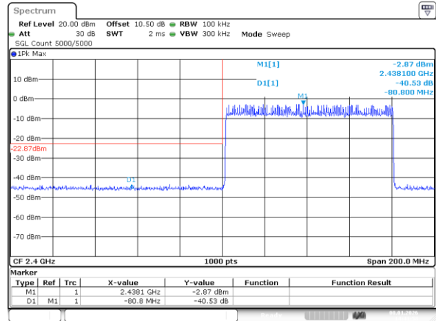
2DH5_Hopping_Lower
