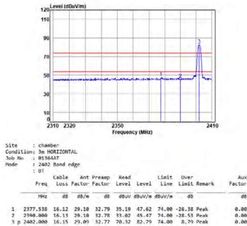
BT_DH5_TX_CH_00_Horizontal
