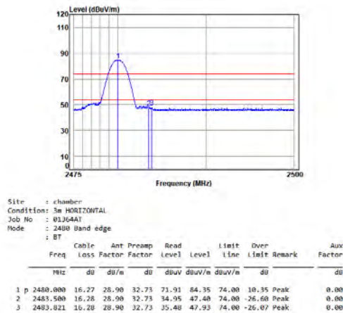
BT_DH5_TX_CH_78_Horizontal
