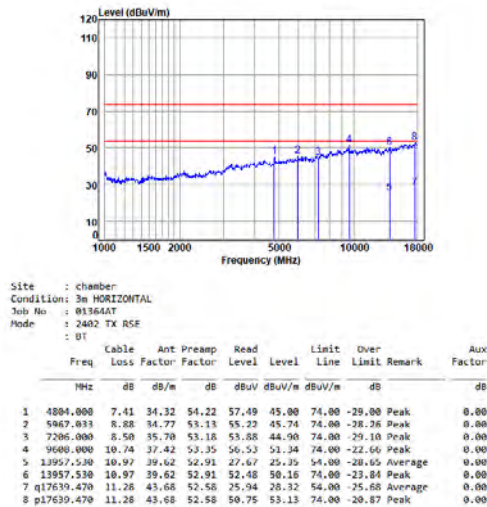
BT_DH5_TX_CH_00_Horizontal
