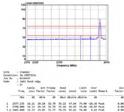
BT_DH5_TX_CH_00_Vertical
