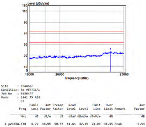
BT_TX_CH_M_Vertical
