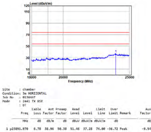
BT_TX_CH_M_Horizontal
