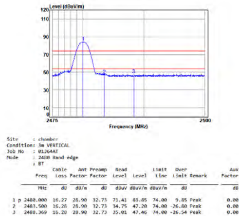
BT_DH5_TX_CH_78_Vertical
