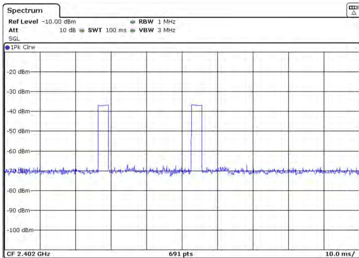
FCC BT DH5 Band edge and RSE TX Worse
