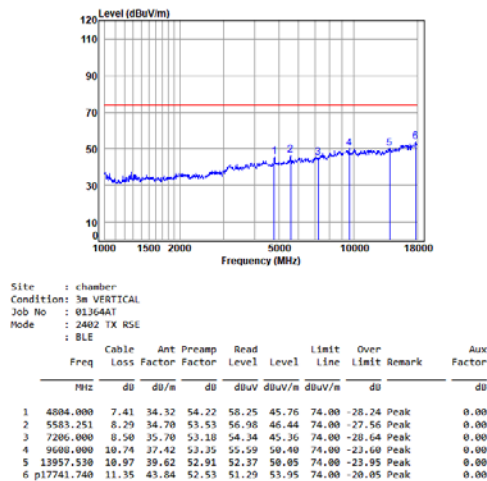
BLE_1M_TX_CH_00_Vertical-Peak
