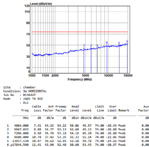
BLE_1M_TX_CH_00_Horizontal-Peak
