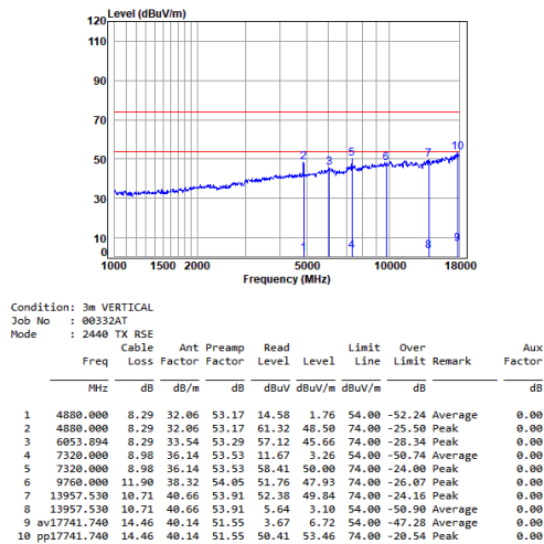
2.4G SRD_TX_CH_M_Vertical
