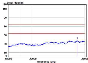
2.4G SRD_TX_CH_M_Horizontal
