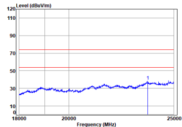
2.4G SRD_TX_CH_M_Vertical
